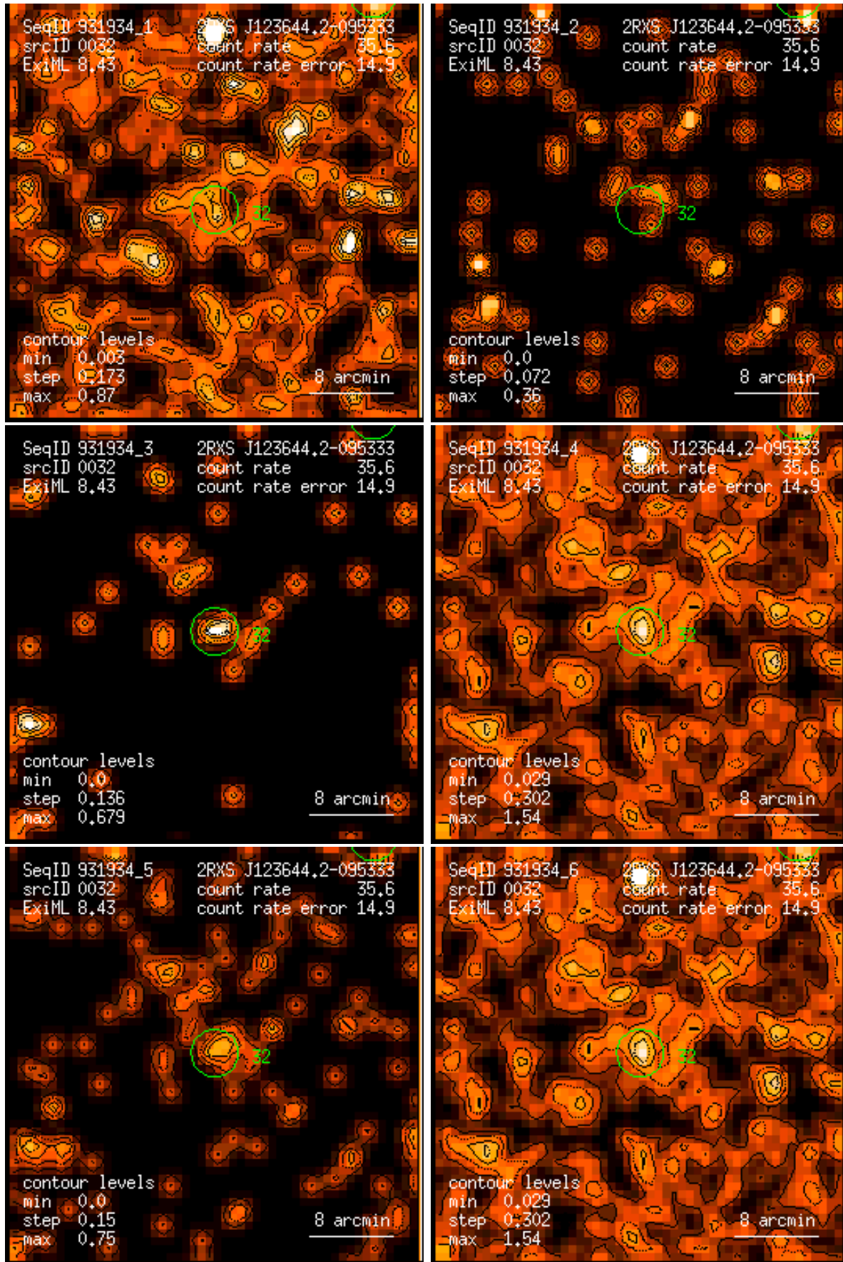
Figure 32: RASS 931934: detection 0032: band rate images, Gaussian filter: (1) PSPC channels 11 – 41, (2) 52 – 90, (3) 91 – 201, (4) 11 – 235, (5) 52 – 201, (6) 11 – 201. Broad band rates in counts/ks. Band rate contour levels in counts/ks/arcmin 2 .
