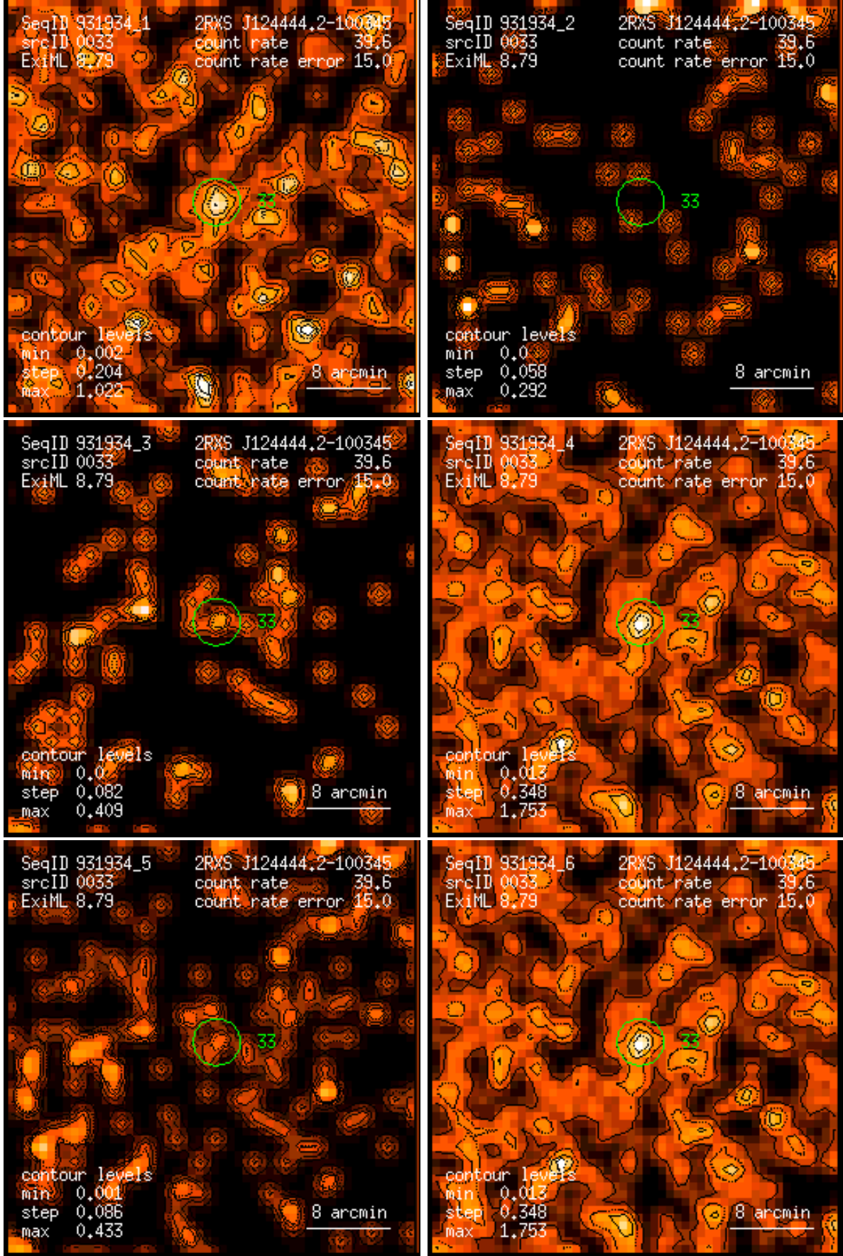
Figure 33: RASS 931934: detection 0033: band rate images, Gaussian filter: (1) PSPC channels 11 – 41, (2) 52 – 90, (3) 91 – 201, (4) 11 – 235, (5) 52 – 201, (6) 11 – 201. Broad band rates in counts/ks. Band rate contour levels in counts/ks/arcmin 2 .
