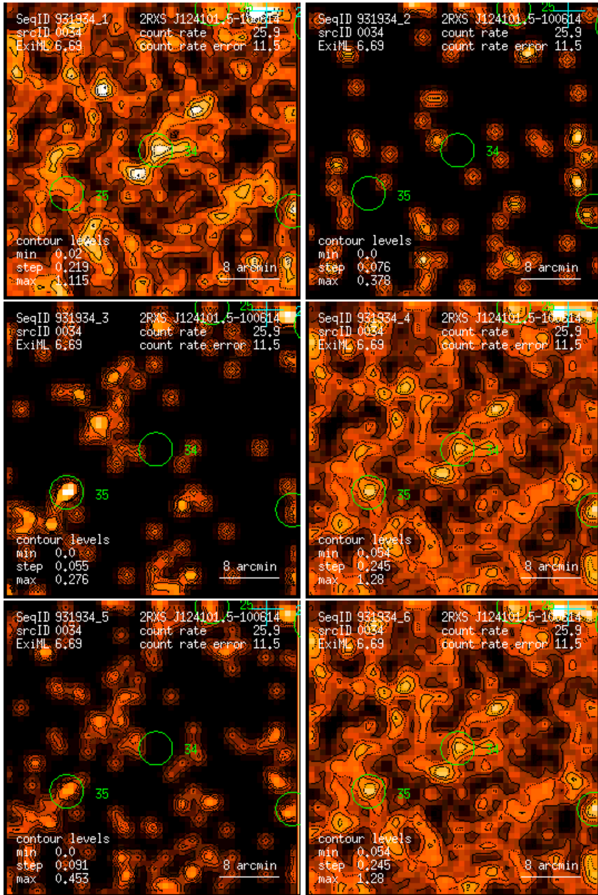
Figure 34: RASS 931934: detection 0034: band rate images, Gaussian filter: (1) PSPC channels 11 – 41, (2) 52 – 90, (3) 91 – 201, (4) 11 – 235, (5) 52 – 201, (6) 11 – 201. Broad band rates in counts/ks. Band rate contour levels in counts/ks/arcmin 2 .
