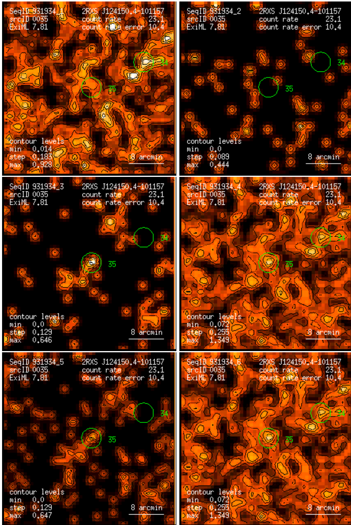
Figure 35: RASS 931934: detection 0035: band rate images, Gaussian filter: (1) PSPC channels 11 – 41, (2) 52 – 90, (3) 91 – 201, (4) 11 – 235, (5) 52 – 201, (6) 11 – 201. Broad band rates in counts/ks. Band rate contour levels in counts/ks/arcmin 2 .
