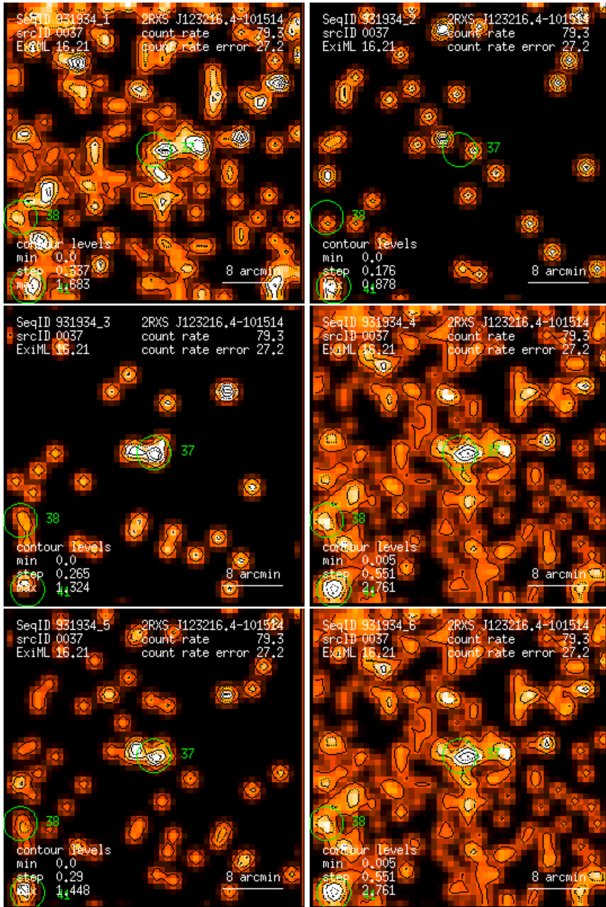
Figure 37: RASS 931934: detection 0037: band rate images, Gaussian filter: (1) PSPC channels 11 – 41, (2) 52 – 90, (3) 91 – 201, (4) 11 – 235, (5) 52 – 201, (6) 11 – 201. Broad band rates in counts/ks. Band rate contour levels in counts/ks/arcmin 2 .
