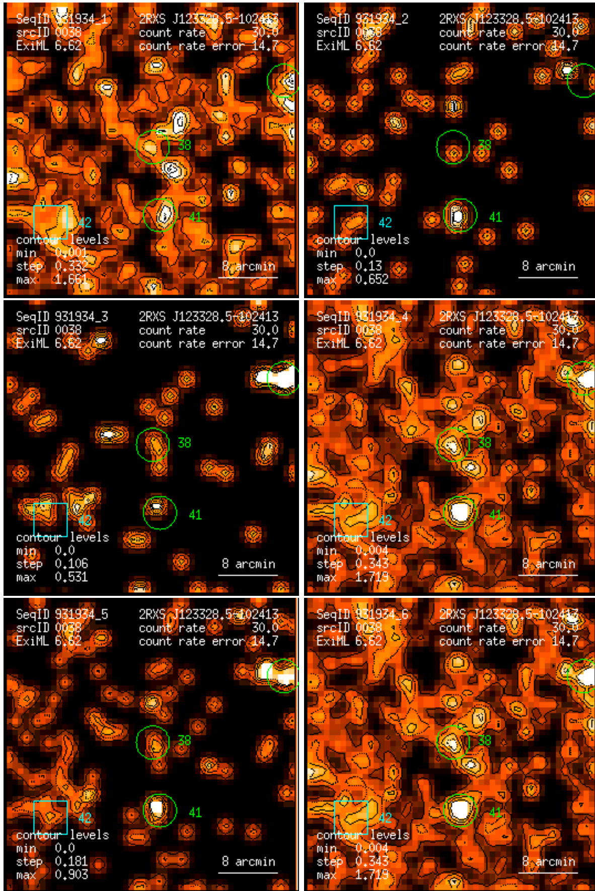
Figure 38: RASS 931934: detection 0038: band rate images, Gaussian filter: (1) PSPC channels 11 – 41, (2) 52 – 90, (3) 91 – 201, (4) 11 – 235, (5) 52 – 201, (6) 11 – 201. Broad band rates in counts/ks. Band rate contour levels in counts/ks/arcmin 2 .
