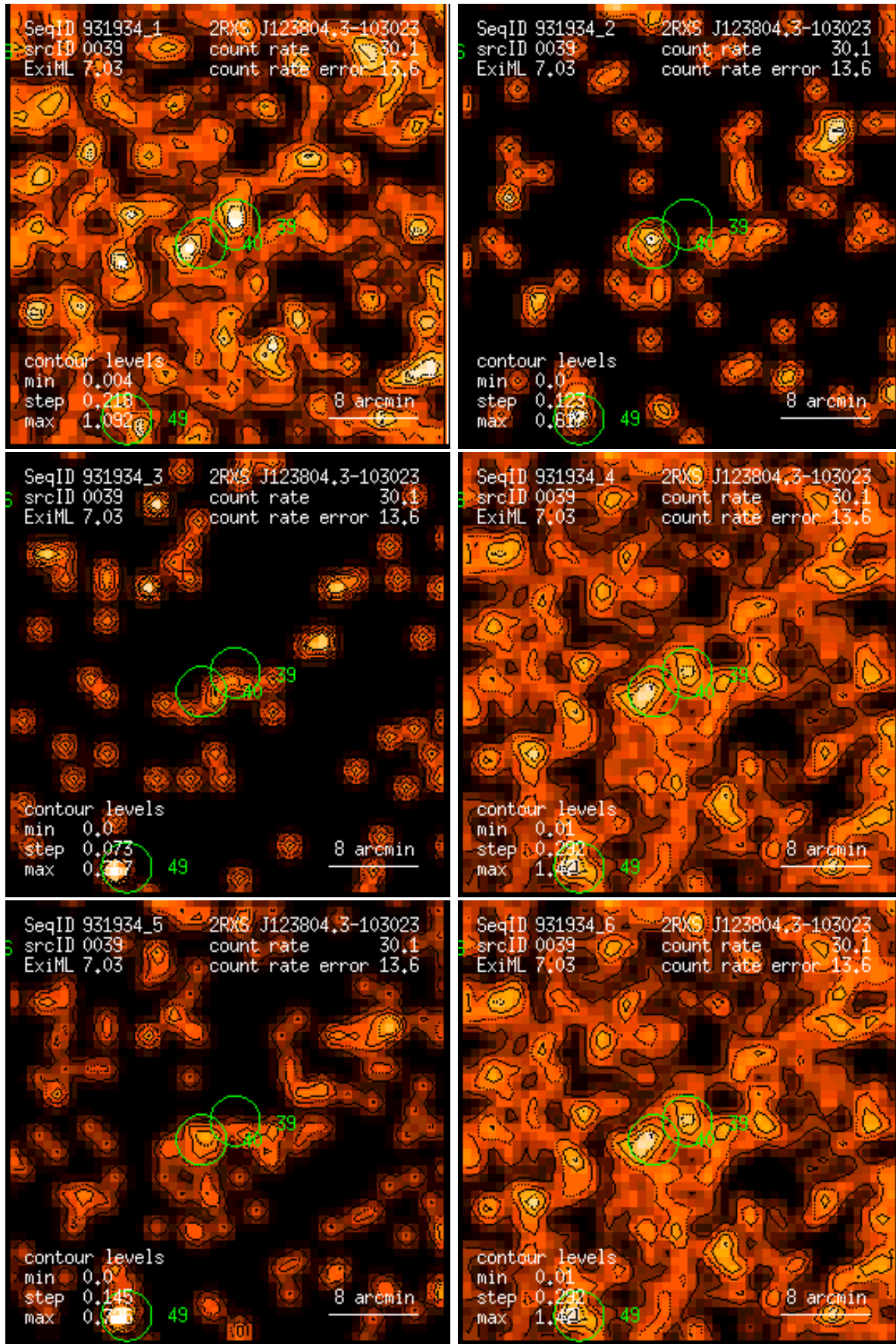
Figure 39: RASS 931934: detection 0039: band rate images, Gaussian filter: (1) PSPC channels 11 – 41, (2) 52 – 90, (3) 91 – 201, (4) 11 – 235, (5) 52 – 201, (6) 11 – 201. Broad band rates in counts/ks. Band rate contour levels in counts/ks/arcmin 2 .
