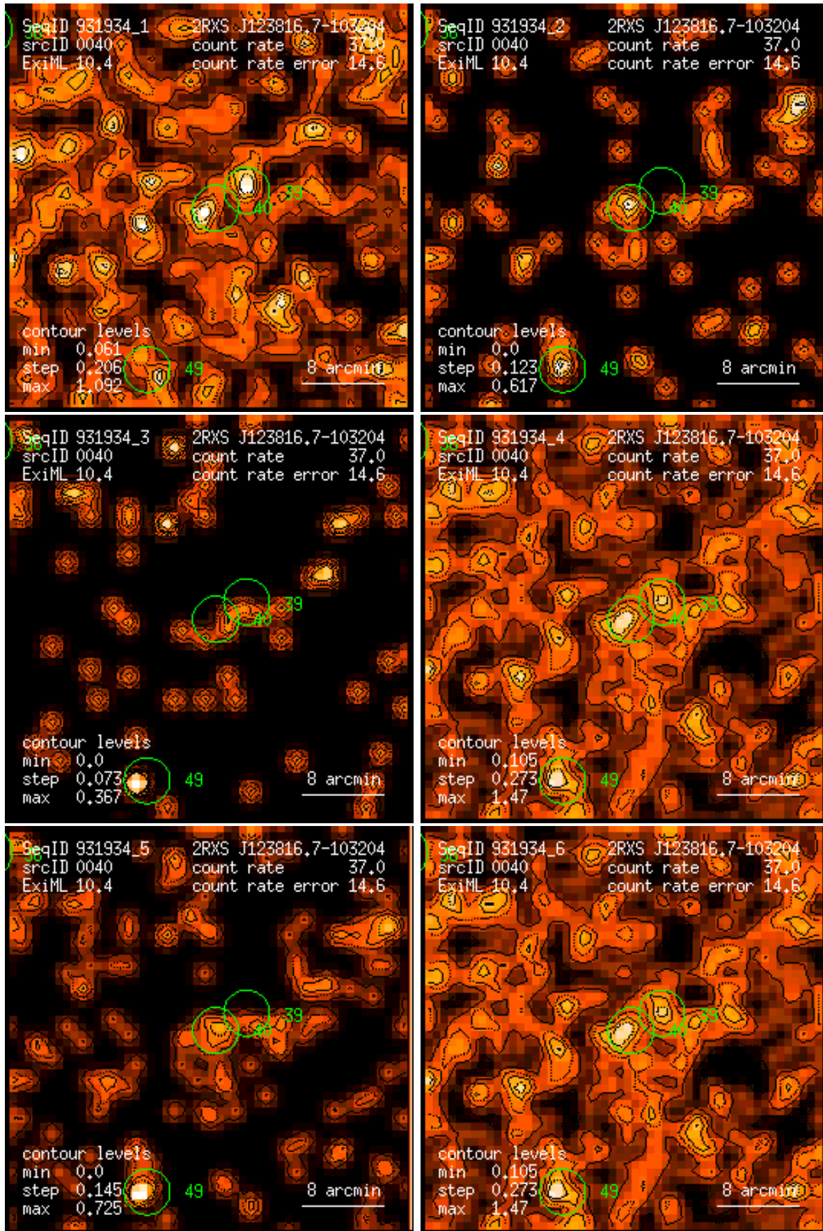
Figure 40: RASS 931934: detection 0040: band rate images, Gaussian filter: (1) PSPC channels 11 – 41, (2) 52 – 90, (3) 91 – 201, (4) 11 – 235, (5) 52 – 201, (6) 11 – 201. Broad band rates in counts/ks. Band rate contour levels in counts/ks/arcmin 2 .
