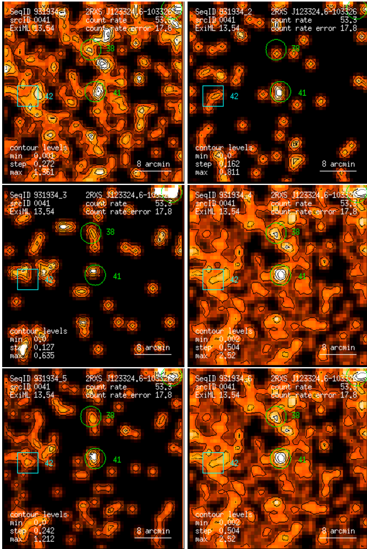
Figure 41: RASS 931934: detection 0041: band rate images, Gaussian filter: (1) PSPC channels 11 – 41, (2) 52 – 90, (3) 91 – 201, (4) 11 – 235, (5) 52 – 201, (6) 11 – 201. Broad band rates in counts/ks. Band rate contour levels in counts/ks/arcmin 2 .
