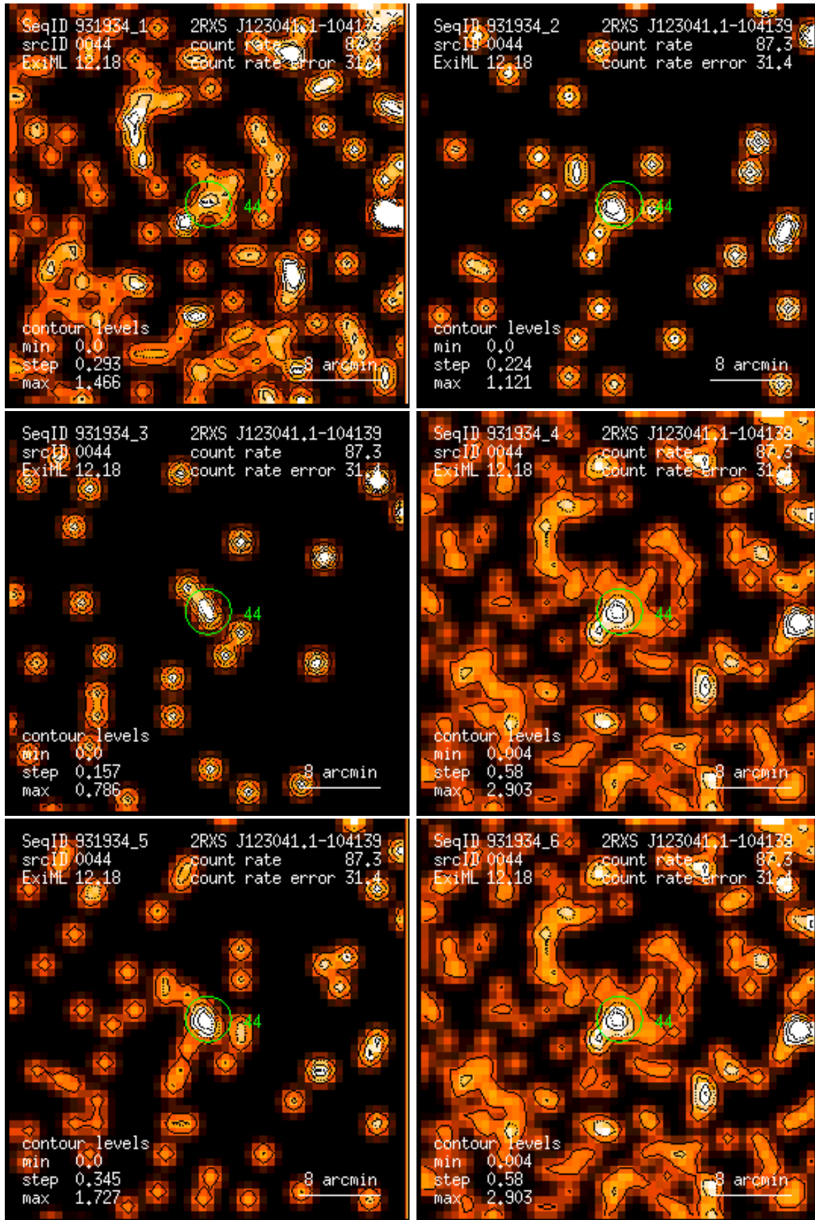
Figure 44: RASS 931934: detection 0044: band rate images, Gaussian filter: (1) PSPC channels 11 – 41, (2) 52 – 90, (3) 91 – 201, (4) 11 – 235, (5) 52 – 201, (6) 11 – 201. Broad band rates in counts/ks. Band rate contour levels in counts/ks/arcmin 2 .
