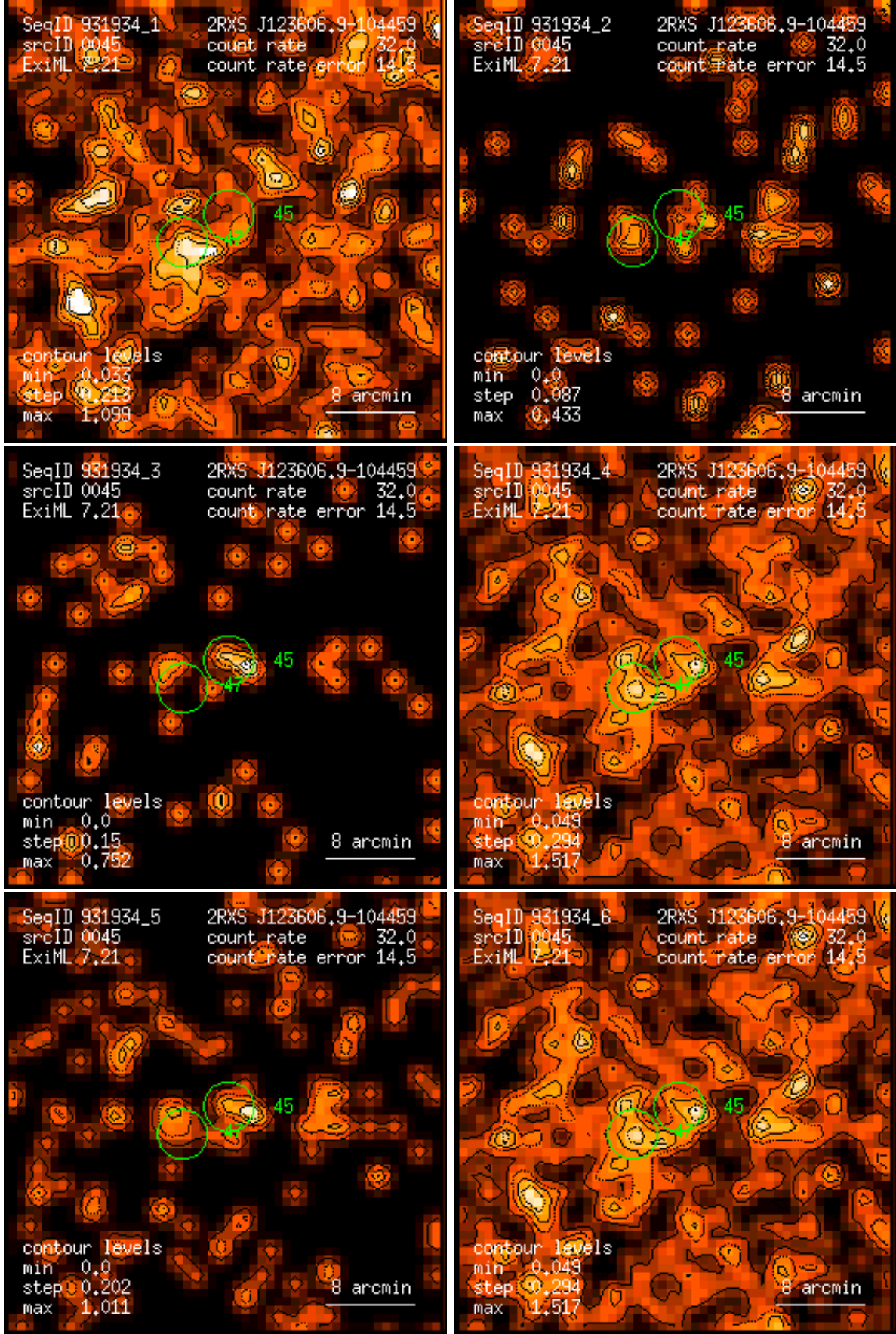
Figure 45: RASS 931934: detection 0045: band rate images, Gaussian filter: (1) PSPC channels 11 – 41, (2) 52 – 90, (3) 91 – 201, (4) 11 – 235, (5) 52 – 201, (6) 11 – 201. Broad band rates in counts/ks. Band rate contour levels in counts/ks/arcmin 2 .
