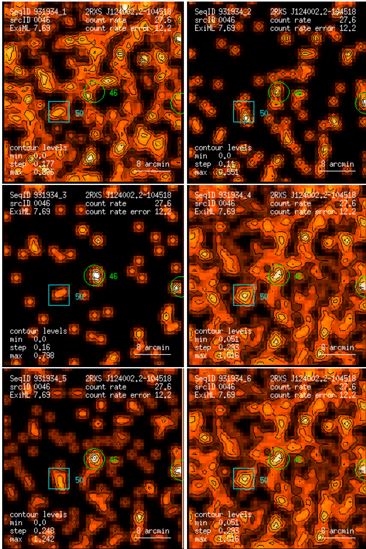
Figure 46: RASS 931934: detection 0046: band rate images, Gaussian filter: (1) PSPC channels 11 – 41, (2) 52 – 90, (3) 91 – 201, (4) 11 – 235, (5) 52 – 201, (6) 11 – 201. Broad band rates in counts/ks. Band rate contour levels in counts/ks/arcmin 2 .
