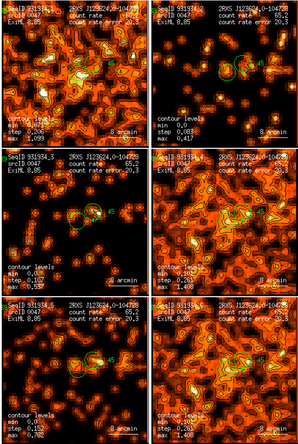
Figure 47: RASS 931934: detection 0047: band rate images, Gaussian filter: (1) PSPC channels 11 – 41, (2) 52 – 90, (3) 91 – 201, (4) 11 – 235, (5) 52 – 201, (6) 11 – 201. Broad band rates in counts/ks. Band rate contour levels in counts/ks/arcmin 2 .
