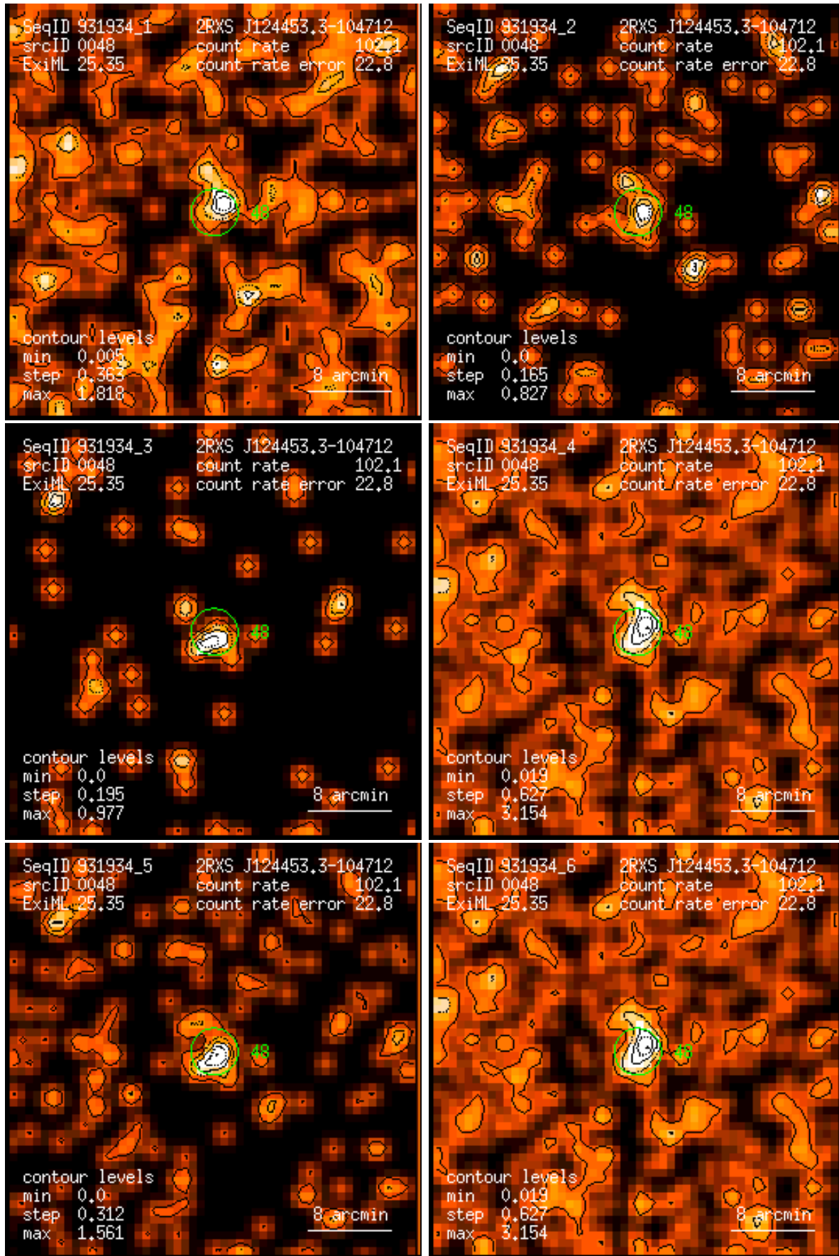
Figure 48: RASS 931934: detection 0048: band rate images, Gaussian filter: (1) PSPC channels 11 – 41, (2) 52 – 90, (3) 91 – 201, (4) 11 – 235, (5) 52 – 201, (6) 11 – 201. Broad band rates in counts/ks. Band rate contour levels in counts/ks/arcmin 2 .
