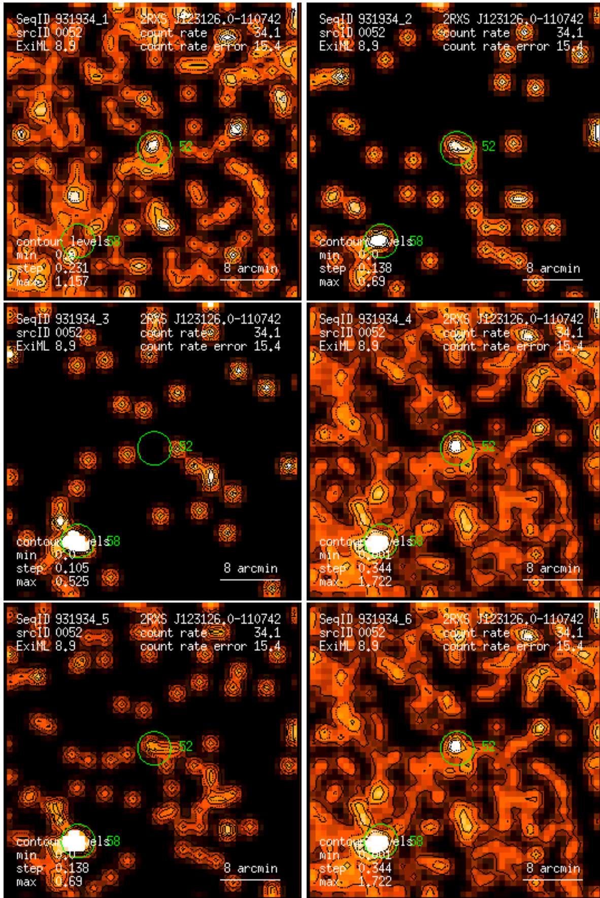
Figure 52: RASS 931934: detection 0052: band rate images, Gaussian filter: (1) PSPC channels 11 – 41, (2) 52 – 90, (3) 91 – 201, (4) 11 – 235, (5) 52 – 201, (6) 11 – 201. Broad band rates in counts/ks. Band rate contour levels in counts/ks/arcmin 2 .
