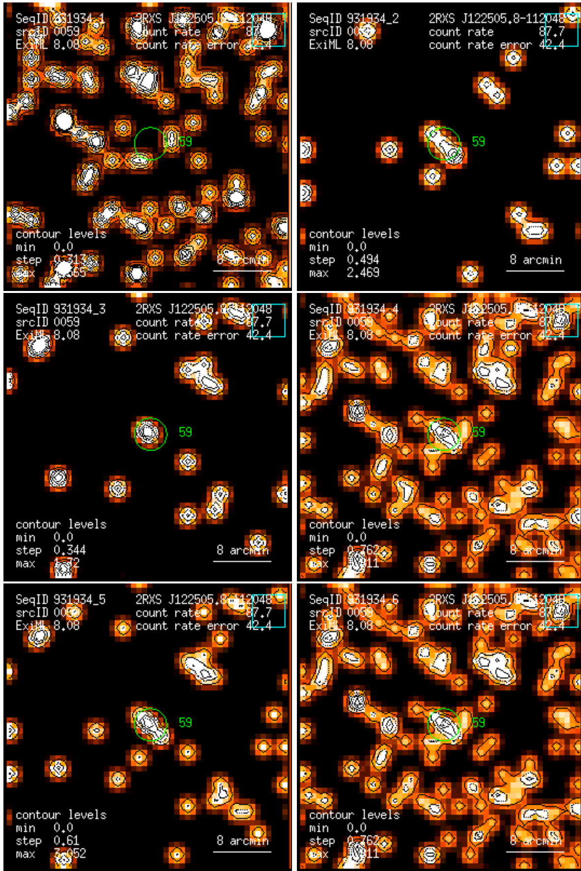
Figure 59: RASS 931934: detection 0059: band rate images, Gaussian filter: (1) PSPC channels 11 – 41, (2) 52 – 90, (3) 91 – 201, (4) 11 – 235, (5) 52 – 201, (6) 11 – 201. Broad band rates in counts/ks. Band rate contour levels in counts/ks/arcmin 2 .
