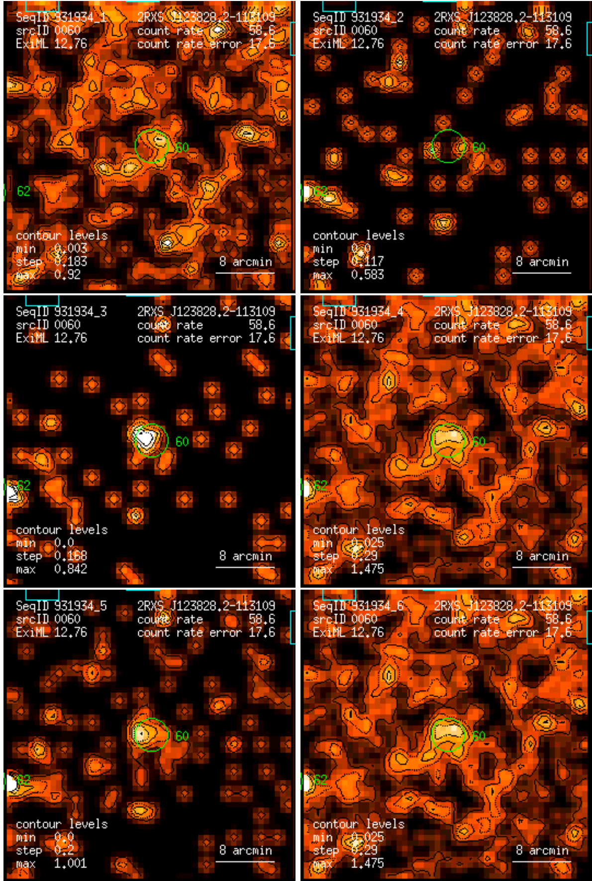
Figure 60: RASS 931934: detection 0060: band rate images, Gaussian filter: (1) PSPC channels 11 – 41, (2) 52 – 90, (3) 91 – 201, (4) 11 – 235, (5) 52 – 201, (6) 11 – 201. Broad band rates in counts/ks. Band rate contour levels in counts/ks/arcmin 2 .
