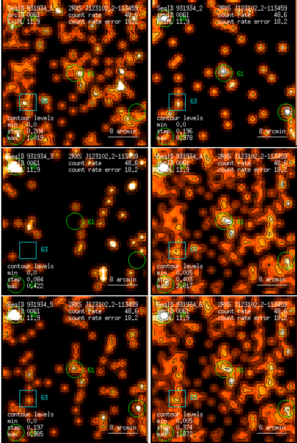
Figure 61: RASS 931934: detection 0061: band rate images, Gaussian filter: (1) PSPC channels 11 – 41, (2) 52 – 90, (3) 91 – 201, (4) 11 – 235, (5) 52 – 201, (6) 11 – 201. Broad band rates in counts/ks. Band rate contour levels in counts/ks/arcmin 2 .
