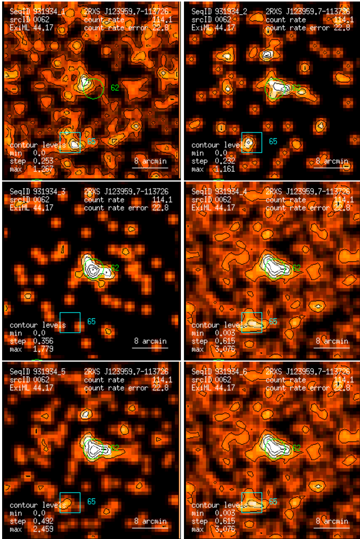
Figure 62: RASS 931934: detection 0062: band rate images, Gaussian filter: (1) PSPC channels 11 – 41, (2) 52 – 90, (3) 91 – 201, (4) 11 – 235, (5) 52 – 201, (6) 11 – 201. Broad band rates in counts/ks. Band rate contour levels in counts/ks/arcmin 2 .
