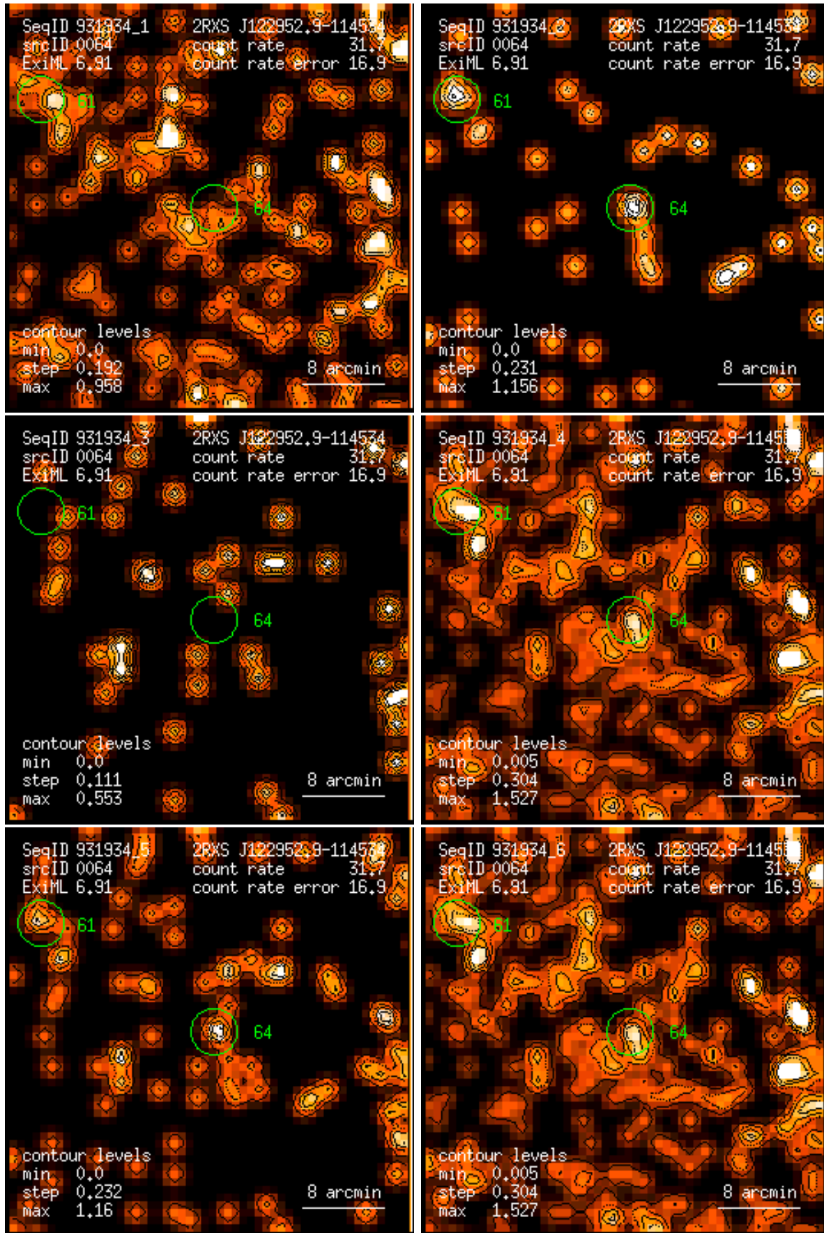
Figure 64: RASS 931934: detection 0064: band rate images, Gaussian filter: (1) PSPC channels 11 – 41, (2) 52 – 90, (3) 91 – 201, (4) 11 – 235, (5) 52 – 201, (6) 11 – 201. Broad band rates in counts/ks. Band rate contour levels in counts/ks/arcmin 2 .
