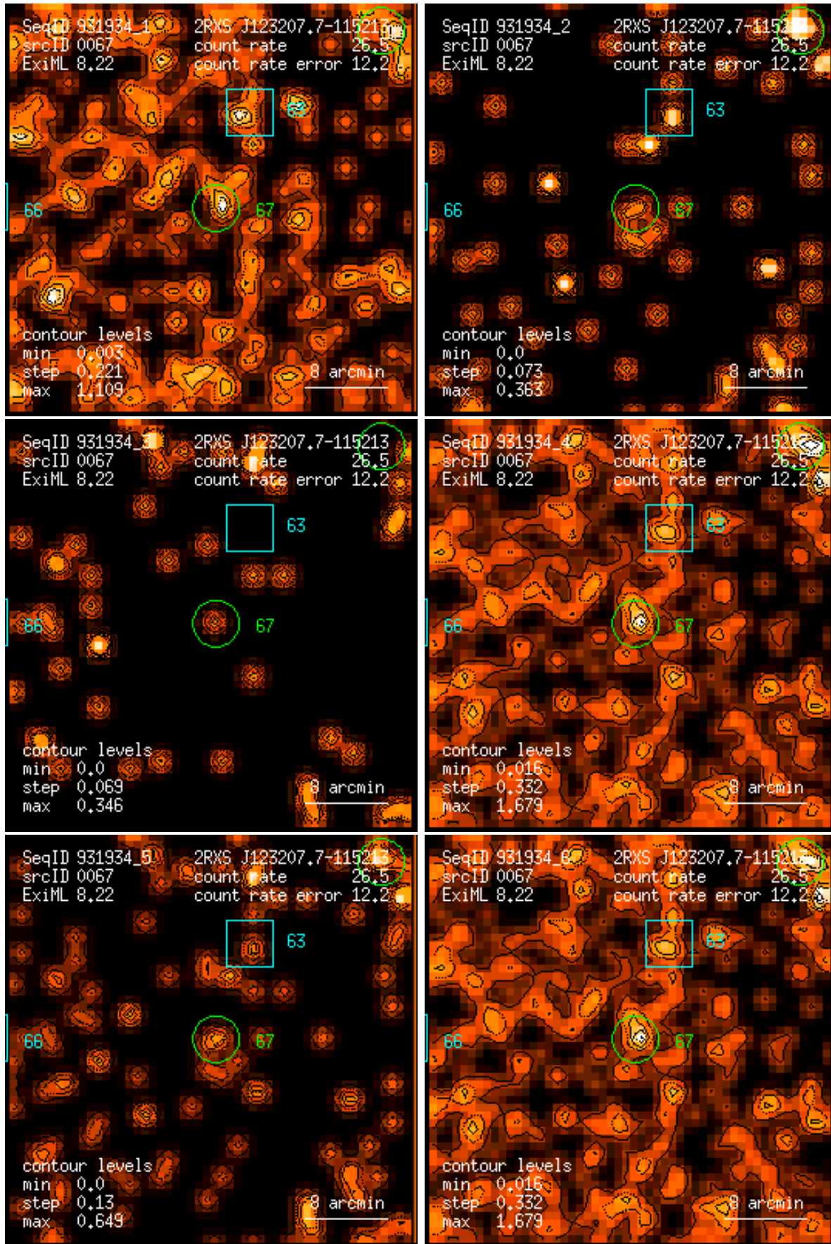
Figure 67: RASS 931934: detection 0067: band rate images, Gaussian filter: (1) PSPC channels 11 – 41, (2) 52 – 90, (3) 91 – 201, (4) 11 – 235, (5) 52 – 201, (6) 11 – 201. Broad band rates in counts/ks. Band rate contour levels in counts/ks/arcmin 2 .
