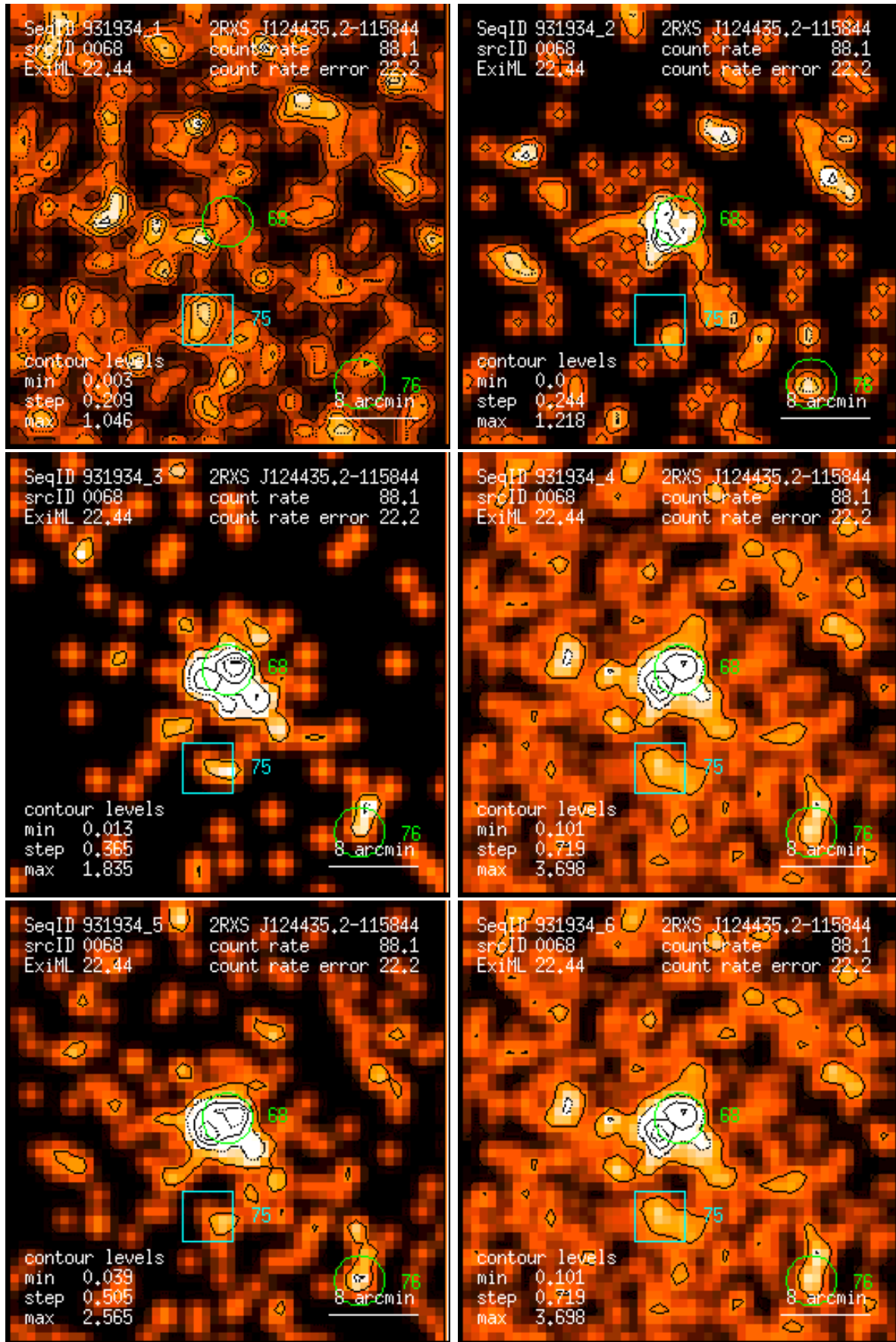
Figure 68: RASS 931934: detection 0068: band rate images, Gaussian filter: (1) PSPC channels 11 – 41, (2) 52 – 90, (3) 91 – 201, (4) 11 – 235, (5) 52 – 201, (6) 11 – 201. Broad band rates in counts/ks. Band rate contour levels in counts/ks/arcmin 2 .
