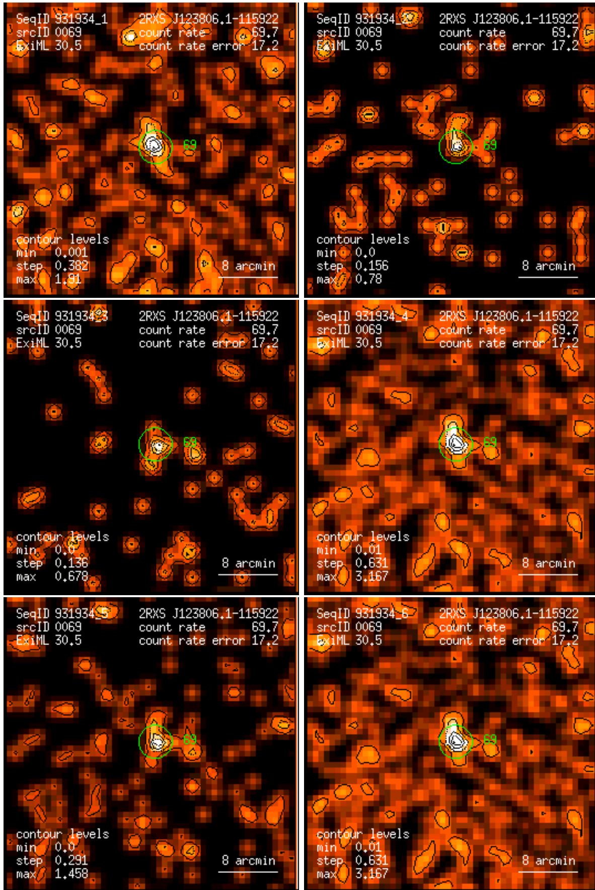
Figure 69: RASS 931934: detection 0069: band rate images, Gaussian filter: (1) PSPC channels 11 – 41, (2) 52 – 90, (3) 91 – 201, (4) 11 – 235, (5) 52 – 201, (6) 11 – 201. Broad band rates in counts/ks. Band rate contour levels in counts/ks/arcmin 2 .
