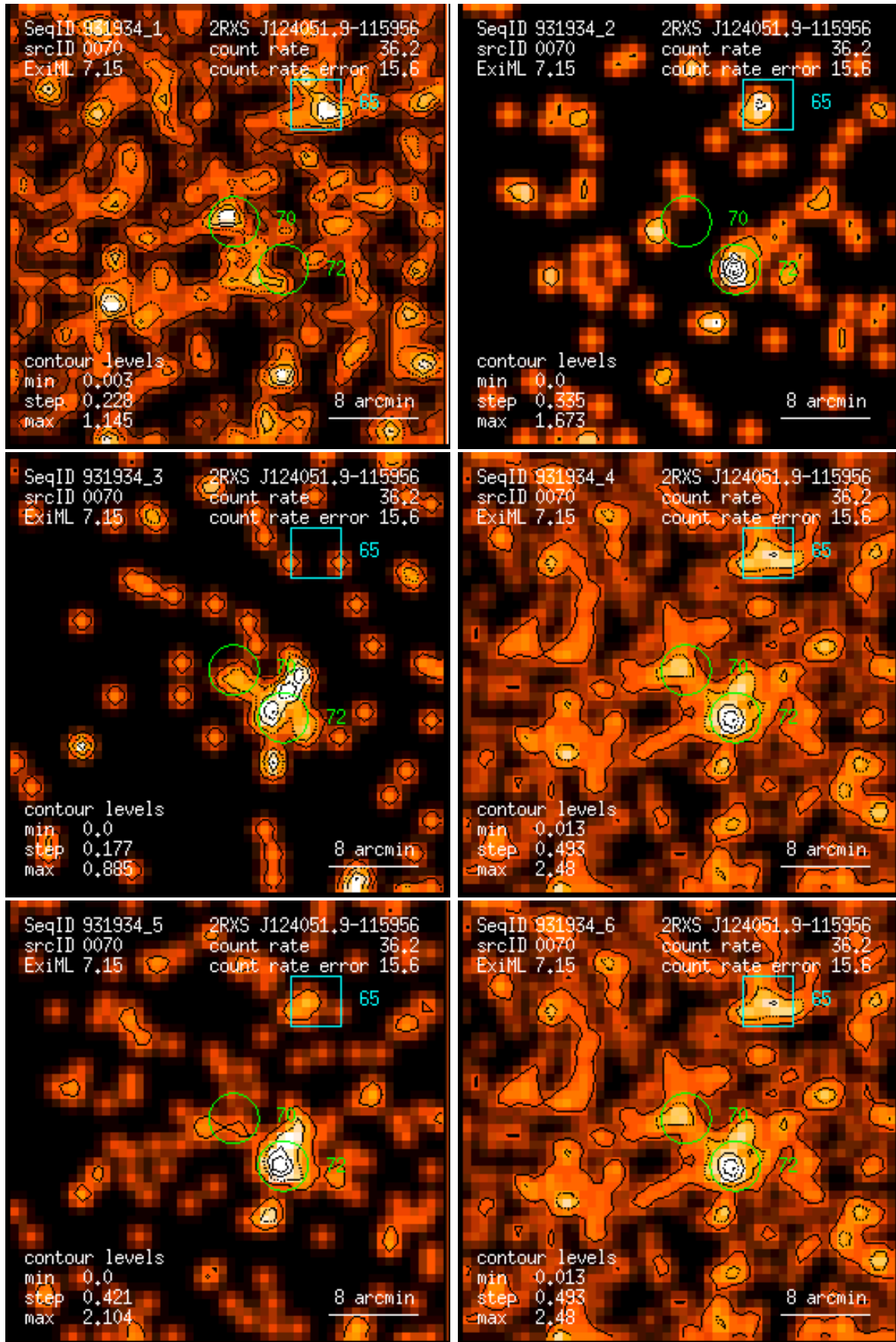
Figure 70: RASS 931934: detection 0070: band rate images, Gaussian filter: (1) PSPC channels 11 – 41, (2) 52 – 90, (3) 91 – 201, (4) 11 – 235, (5) 52 – 201, (6) 11 – 201. Broad band rates in counts/ks. Band rate contour levels in counts/ks/arcmin 2 .
