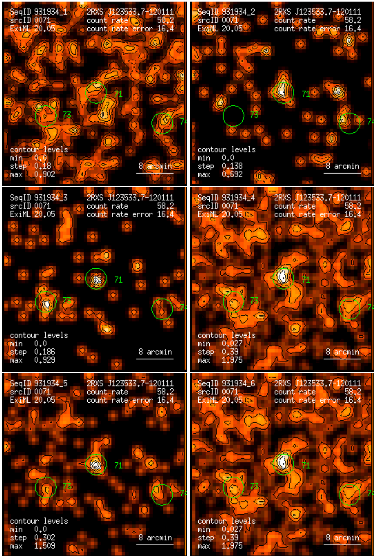
Figure 71: RASS 931934: detection 0071: band rate images, Gaussian filter: (1) PSPC channels 11 – 41, (2) 52 – 90, (3) 91 – 201, (4) 11 – 235, (5) 52 – 201, (6) 11 – 201. Broad band rates in counts/ks. Band rate contour levels in counts/ks/arcmin 2 .
