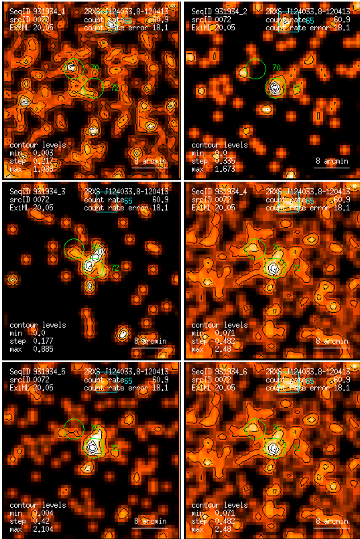
Figure 72: RASS 931934: detection 0072: band rate images, Gaussian filter: (1) PSPC channels 11 – 41, (2) 52 – 90, (3) 91 – 201, (4) 11 – 235, (5) 52 – 201, (6) 11 – 201. Broad band rates in counts/ks. Band rate contour levels in counts/ks/arcmin 2 .
