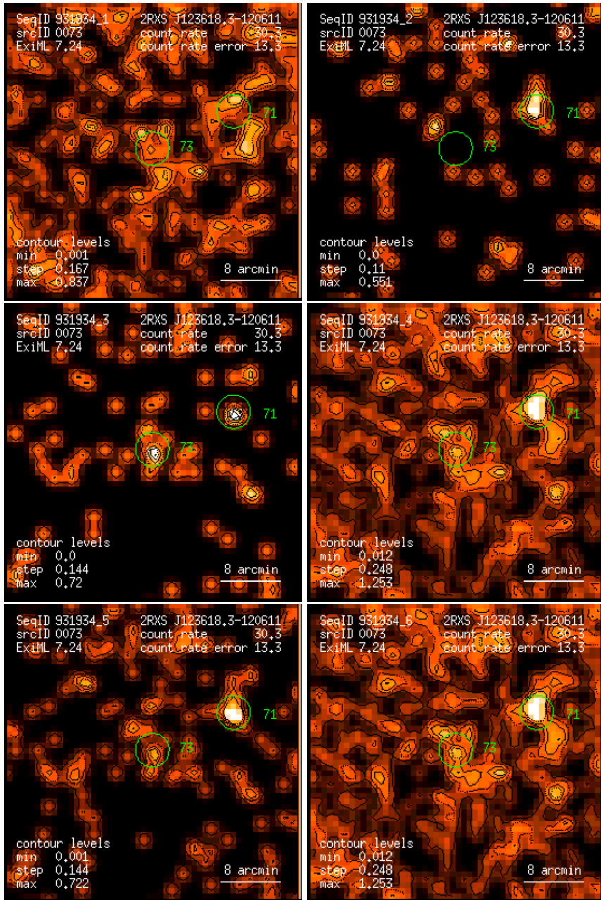
Figure 73: RASS 931934: detection 0073: band rate images, Gaussian filter: (1) PSPC channels 11 – 41, (2) 52 – 90, (3) 91 – 201, (4) 11 – 235, (5) 52 – 201, (6) 11 – 201. Broad band rates in counts/ks. Band rate contour levels in counts/ks/arcmin 2 .
