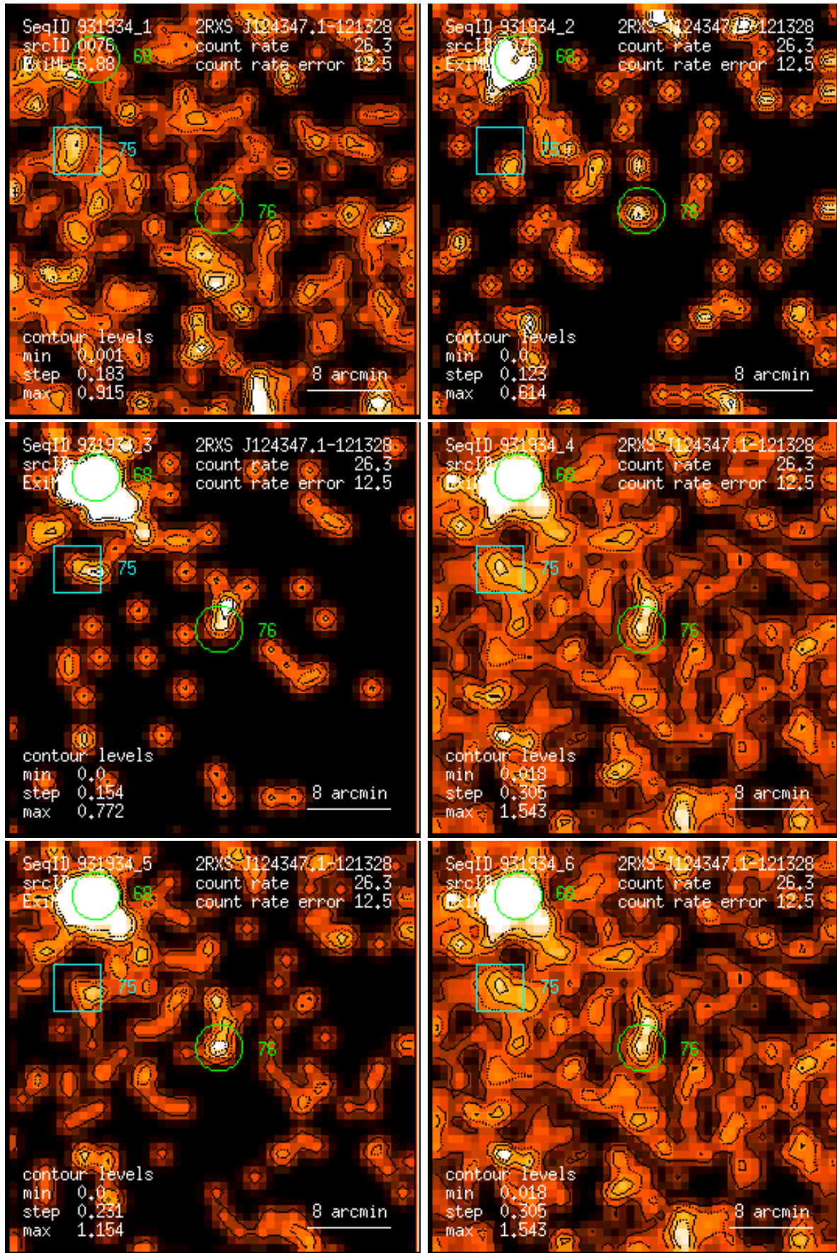
Figure 76: RASS 931934: detection 0076: band rate images, Gaussian filter: (1) PSPC channels 11 – 41, (2) 52 – 90, (3) 91 – 201, (4) 11 – 235, (5) 52 – 201, (6) 11 – 201. Broad band rates in counts/ks. Band rate contour levels in counts/ks/arcmin 2 .
