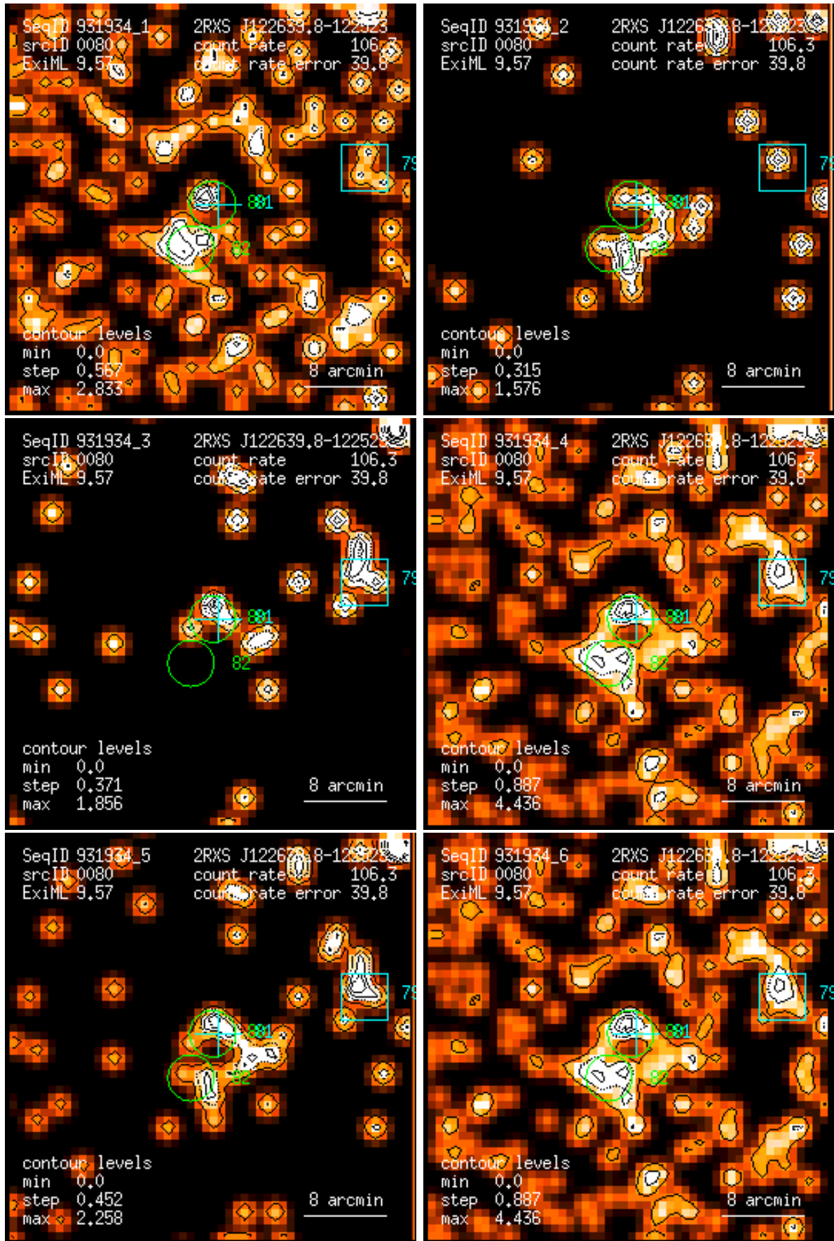
Figure 80: RASS 931934: detection 0080: band rate images, Gaussian filter: (1) PSPC channels 11 – 41, (2) 52 – 90, (3) 91 – 201, (4) 11 – 235, (5) 52 – 201, (6) 11 – 201. Broad band rates in counts/ks. Band rate contour levels in counts/ks/arcmin 2 .
