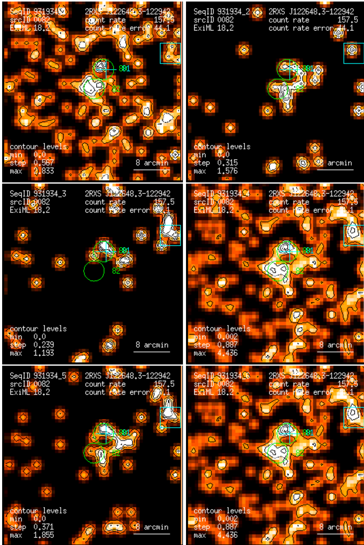
Figure 82: RASS 931934: detection 0082: band rate images, Gaussian filter: (1) PSPC channels 11 – 41, (2) 52 – 90, (3) 91 – 201, (4) 11 – 235, (5) 52 – 201, (6) 11 – 201. Broad band rates in counts/ks. Band rate contour levels in counts/ks/arcmin 2 .
