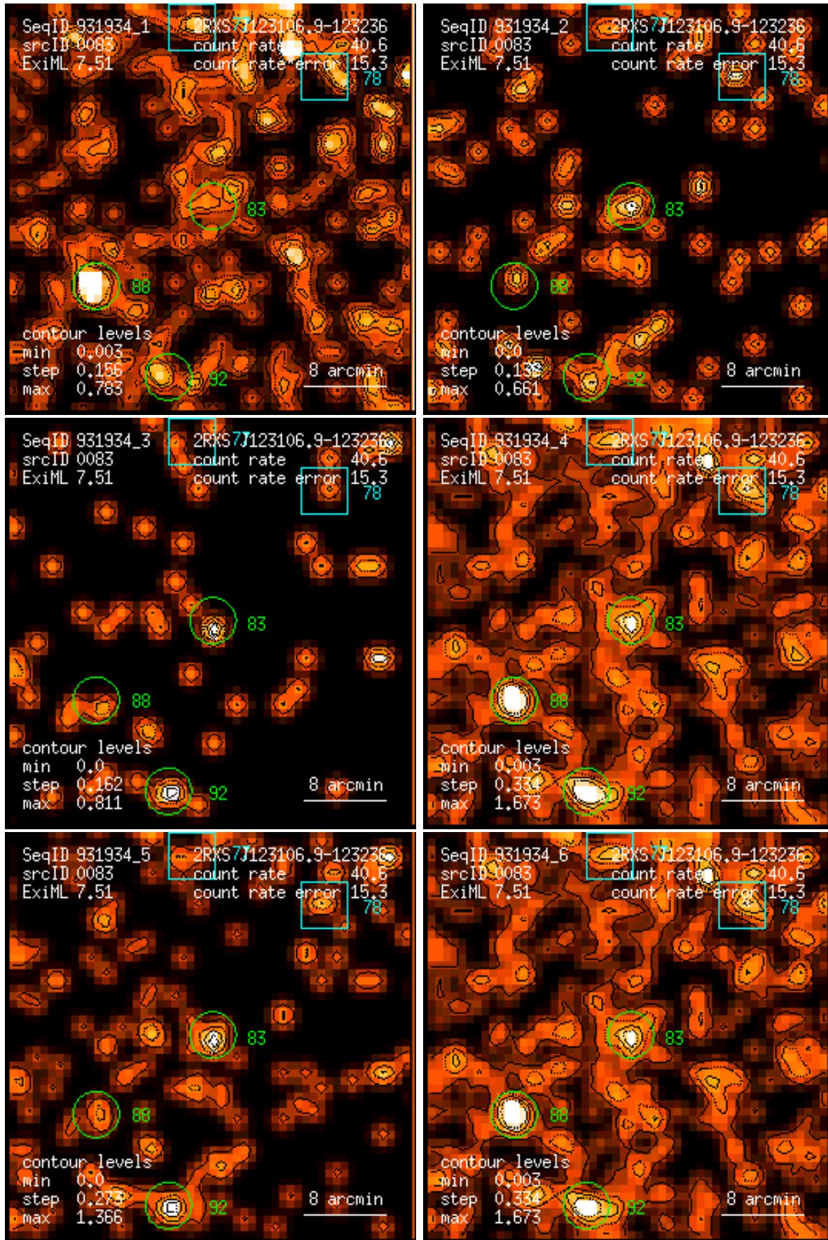
Figure 83: RASS 931934: detection 0083: band rate images, Gaussian filter: (1) PSPC channels 11 – 41, (2) 52 – 90, (3) 91 – 201, (4) 11 – 235, (5) 52 – 201, (6) 11 – 201. Broad band rates in counts/ks. Band rate contour levels in counts/ks/arcmin 2 .
