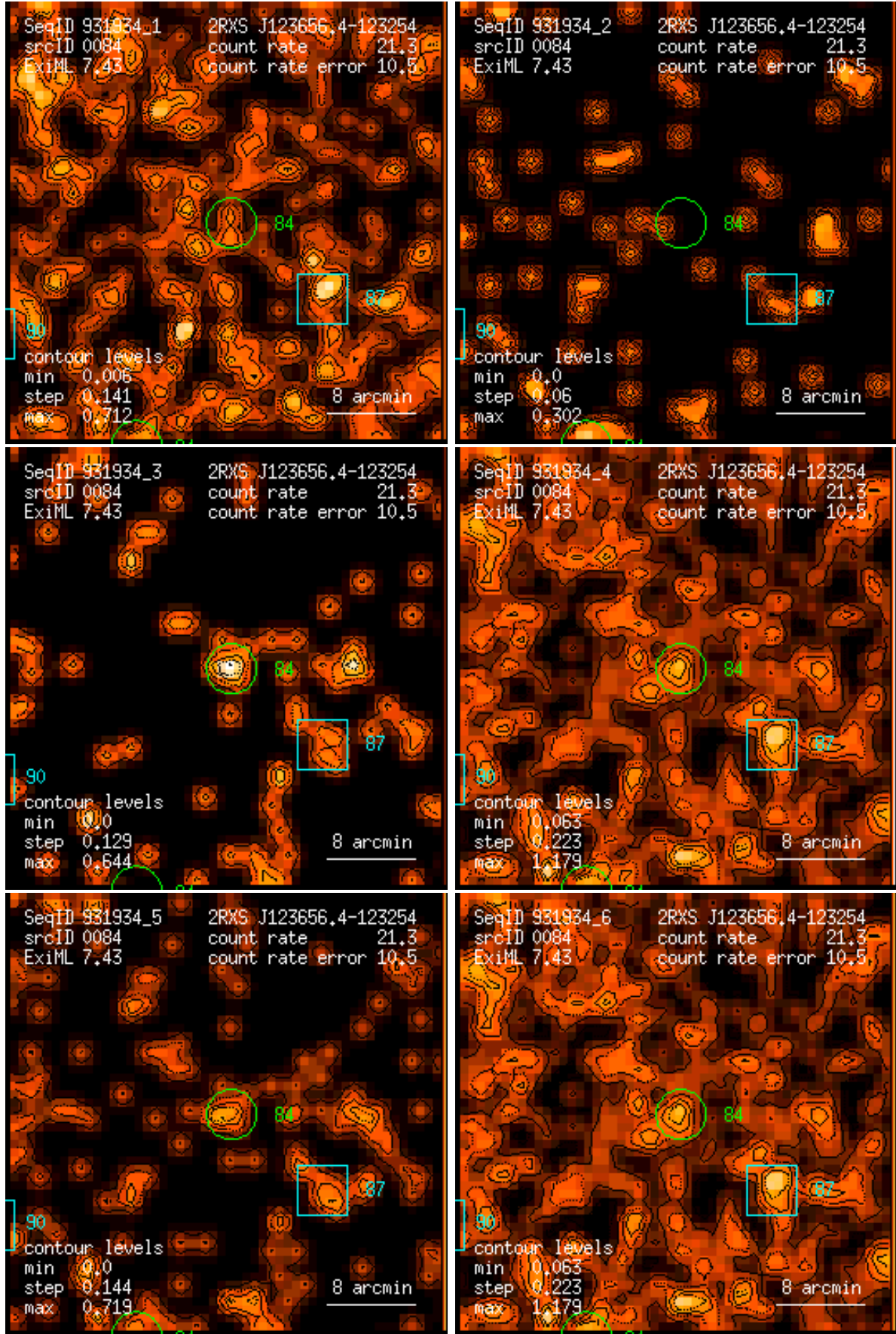
Figure 84: RASS 931934: detection 0084: band rate images, Gaussian filter: (1) PSPC channels 11 – 41, (2) 52 – 90, (3) 91 – 201, (4) 11 – 235, (5) 52 – 201, (6) 11 – 201. Broad band rates in counts/ks. Band rate contour levels in counts/ks/arcmin 2 .
