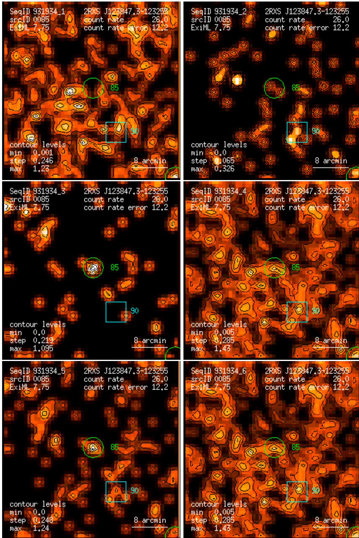
Figure 85: RASS 931934: detection 0085: band rate images, Gaussian filter: (1) PSPC channels 11 – 41, (2) 52 – 90, (3) 91 – 201, (4) 11 – 235, (5) 52 – 201, (6) 11 – 201. Broad band rates in counts/ks. Band rate contour levels in counts/ks/arcmin 2 .
