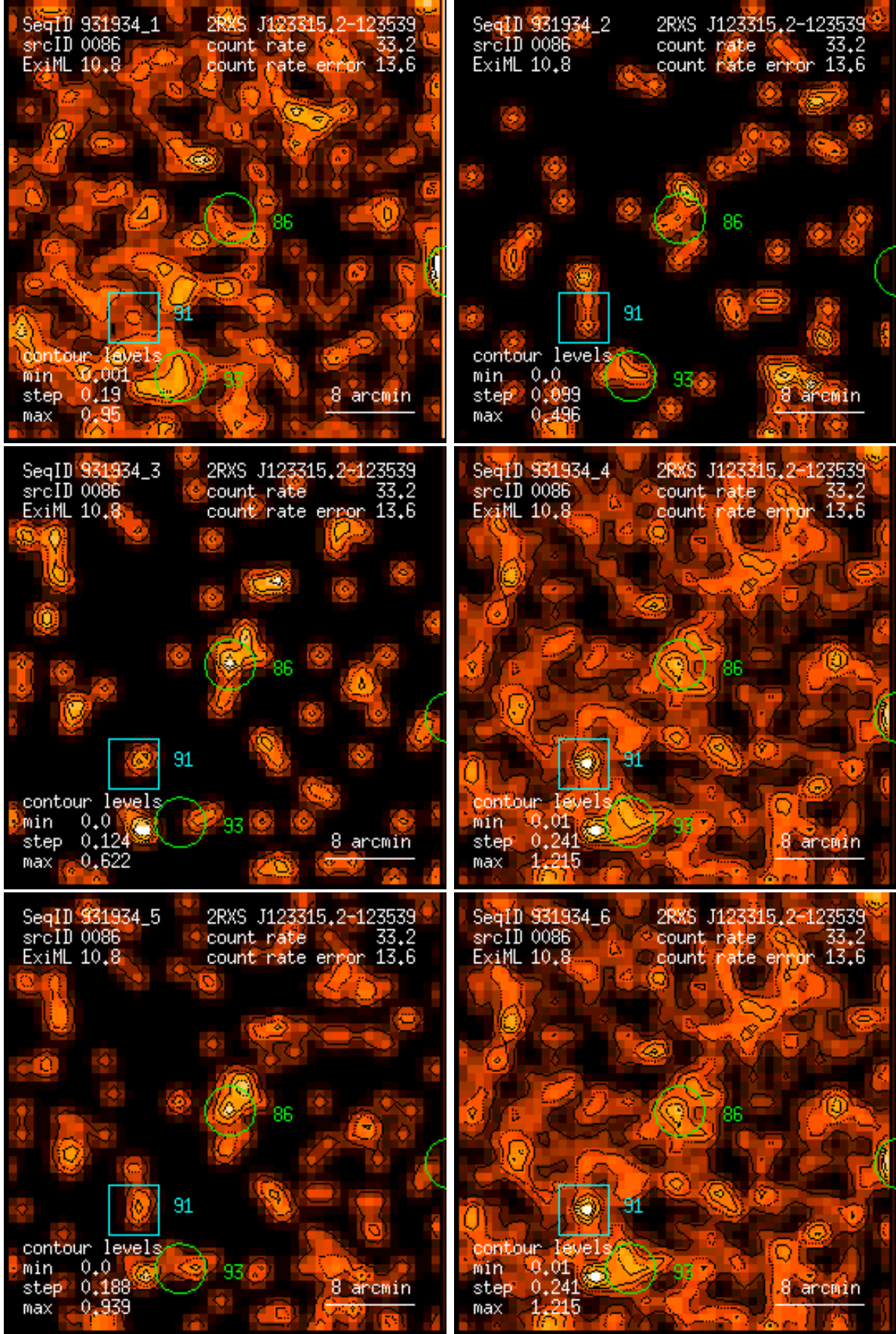
Figure 86: RASS 931934: detection 0086: band rate images, Gaussian filter: (1) PSPC channels 11 – 41, (2) 52 – 90, (3) 91 – 201, (4) 11 – 235, (5) 52 – 201, (6) 11 – 201. Broad band rates in counts/ks. Band rate contour levels in counts/ks/arcmin 2 .
