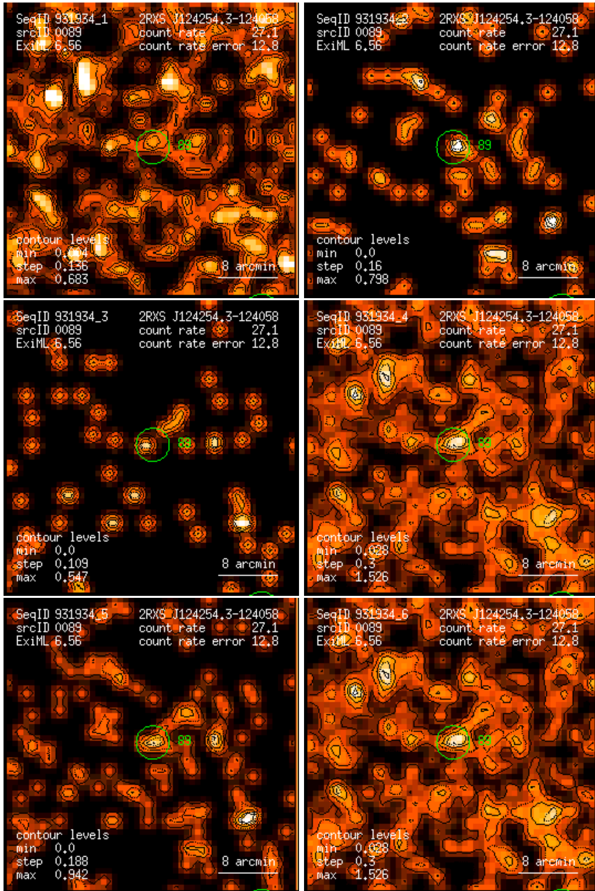
Figure 89: RASS 931934: detection 0089: band rate images, Gaussian filter: (1) PSPC channels 11 – 41, (2) 52 – 90, (3) 91 – 201, (4) 11 – 235, (5) 52 – 201, (6) 11 – 201. Broad band rates in counts/ks. Band rate contour levels in counts/ks/arcmin 2 .
