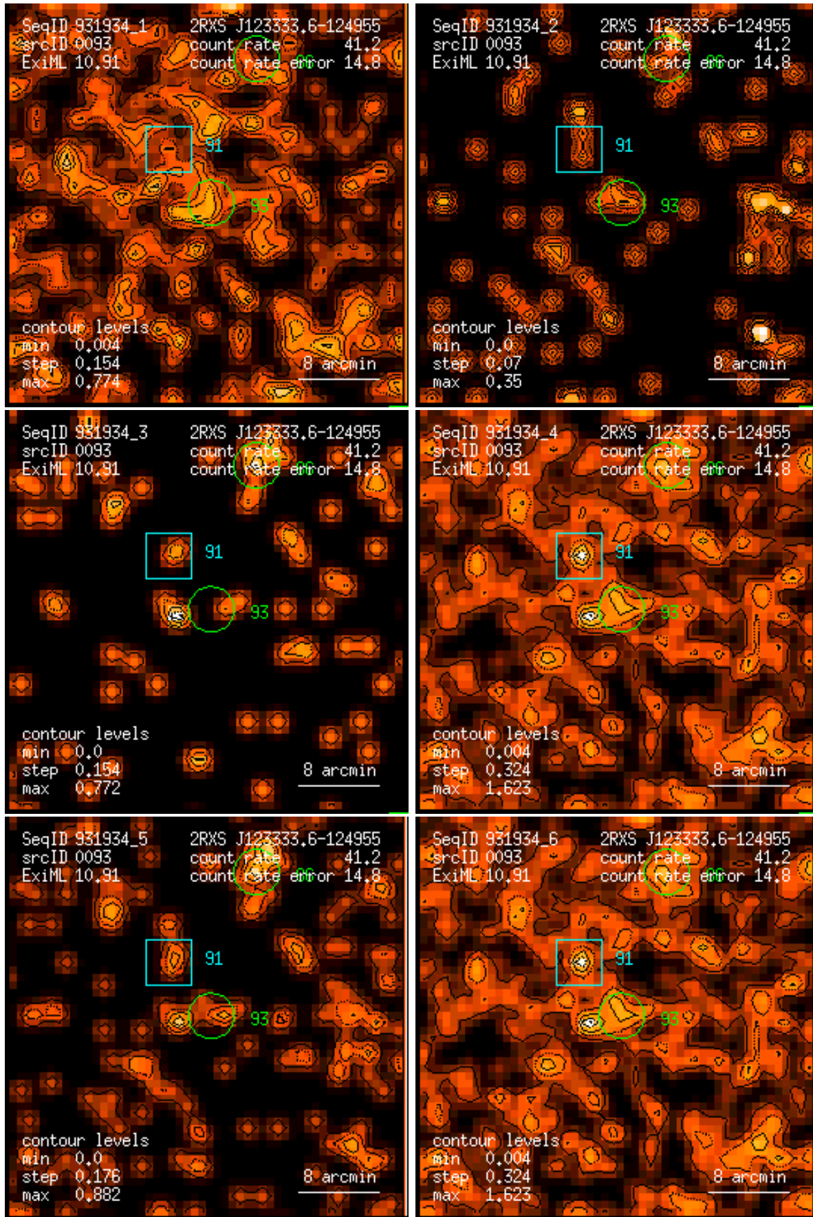
Figure 93: RASS 931934: detection 0093: band rate images, Gaussian filter: (1) PSPC channels 11 – 41, (2) 52 – 90, (3) 91 – 201, (4) 11 – 235, (5) 52 – 201, (6) 11 – 201. Broad band rates in counts/ks. Band rate contour levels in counts/ks/arcmin 2 .
