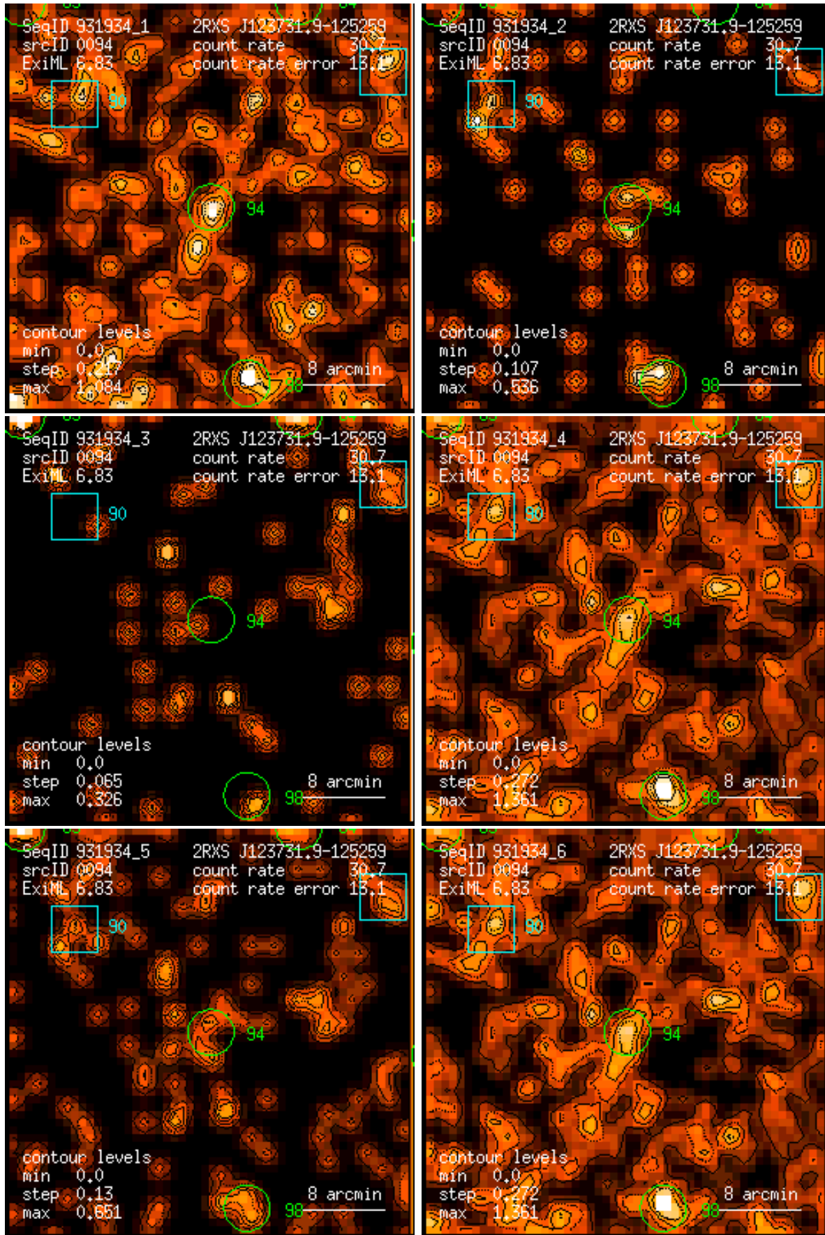
Figure 94: RASS 931934: detection 0094: band rate images, Gaussian filter: (1) PSPC channels 11 – 41, (2) 52 – 90, (3) 91 – 201, (4) 11 – 235, (5) 52 – 201, (6) 11 – 201. Broad band rates in counts/ks. Band rate contour levels in counts/ks/arcmin 2 .
