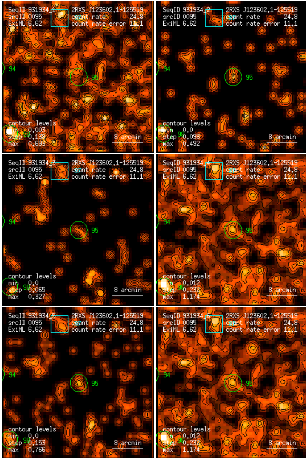
Figure 95: RASS 931934: detection 0095: band rate images, Gaussian filter: (1) PSPC channels 11 – 41, (2) 52 – 90, (3) 91 – 201, (4) 11 – 235, (5) 52 – 201, (6) 11 – 201. Broad band rates in counts/ks. Band rate contour levels in counts/ks/arcmin 2 .
