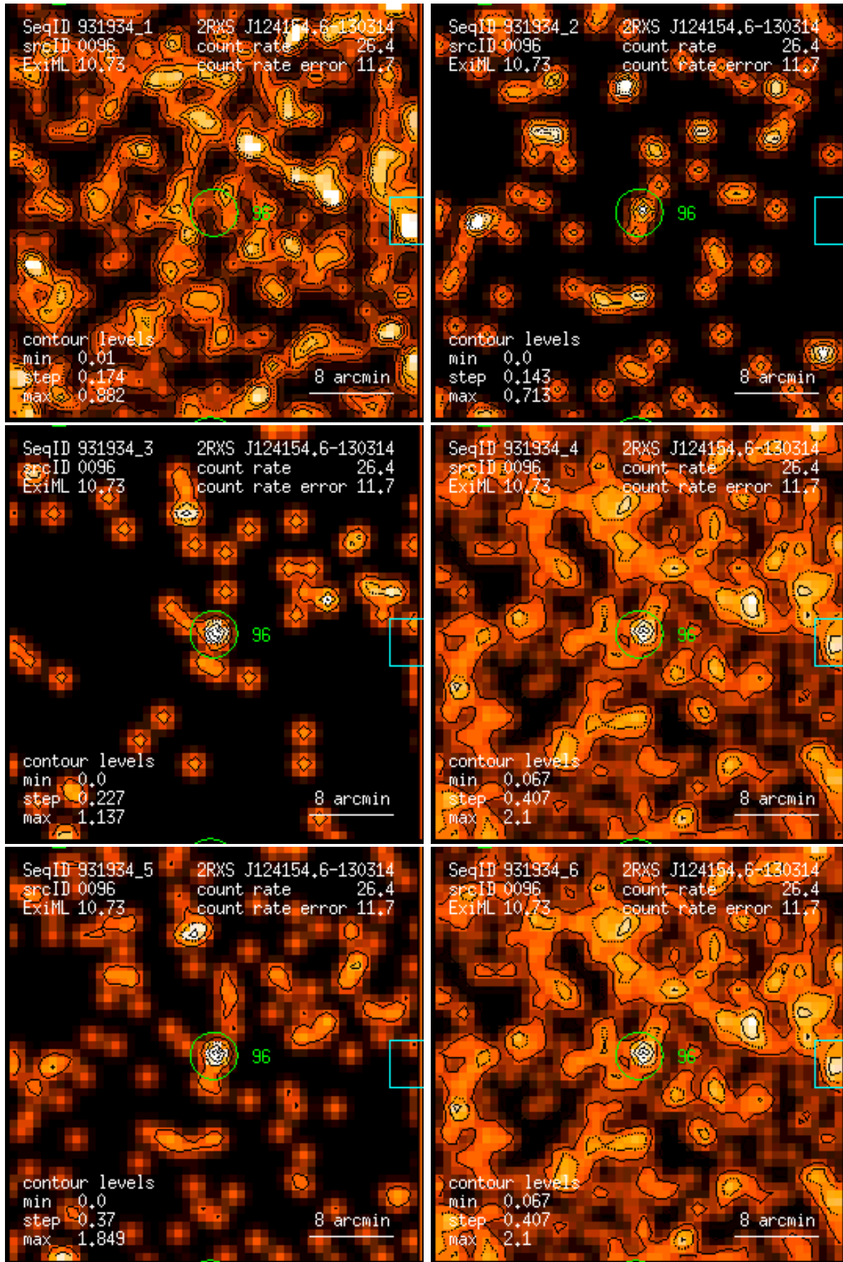
Figure 96: RASS 931934: detection 0096: band rate images, Gaussian filter: (1) PSPC channels 11 – 41, (2) 52 – 90, (3) 91 – 201, (4) 11 – 235, (5) 52 – 201, (6) 11 – 201. Broad band rates in counts/ks. Band rate contour levels in counts/ks/arcmin 2 .
