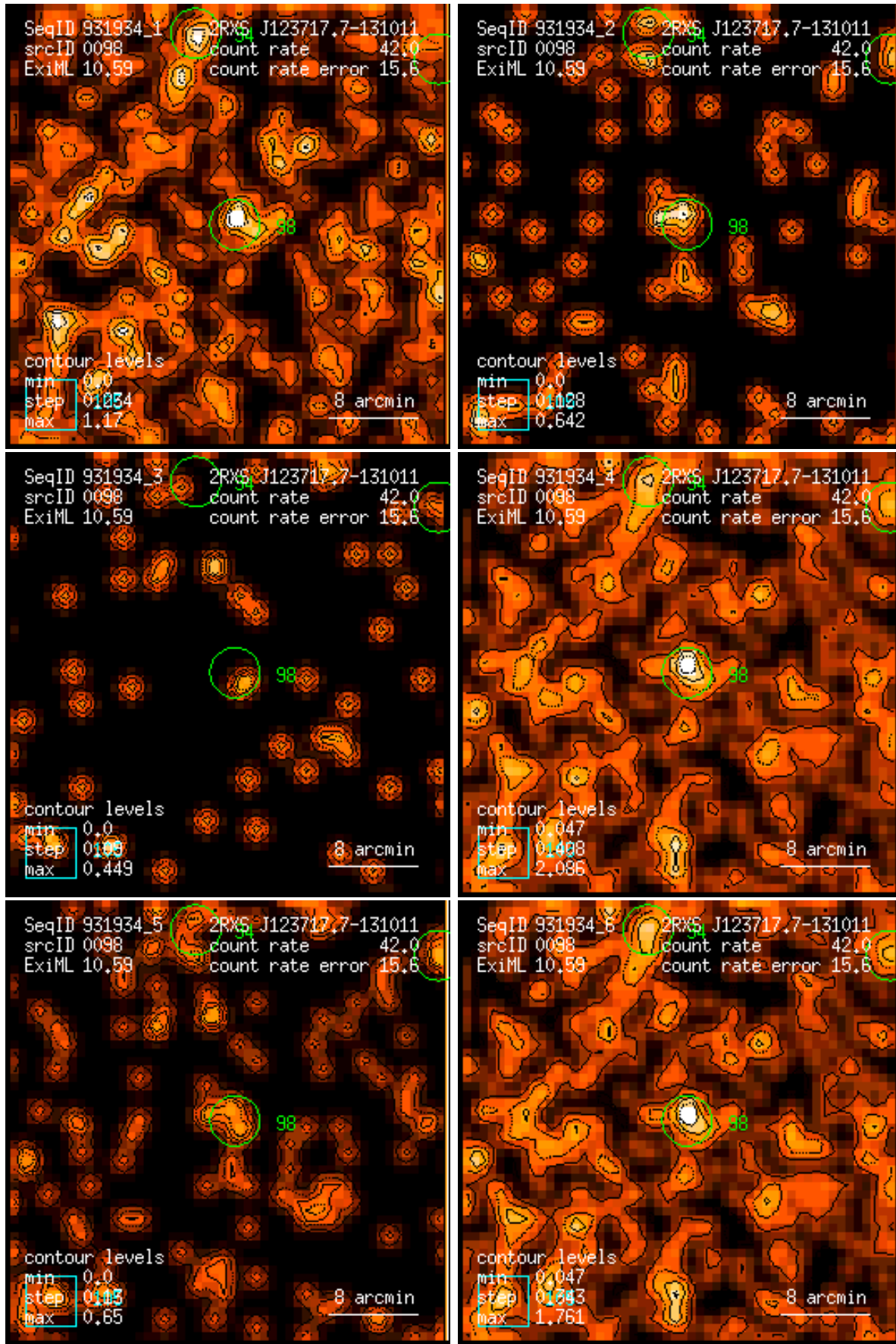
Figure 98: RASS 931934: detection 0098: band rate images, Gaussian filter: (1) PSPC channels 11 – 41, (2) 52 – 90, (3) 91 – 201, (4) 11 – 235, (5) 52 – 201, (6) 11 – 201. Broad band rates in counts/ks. Band rate contour levels in counts/ks/arcmin 2 .
