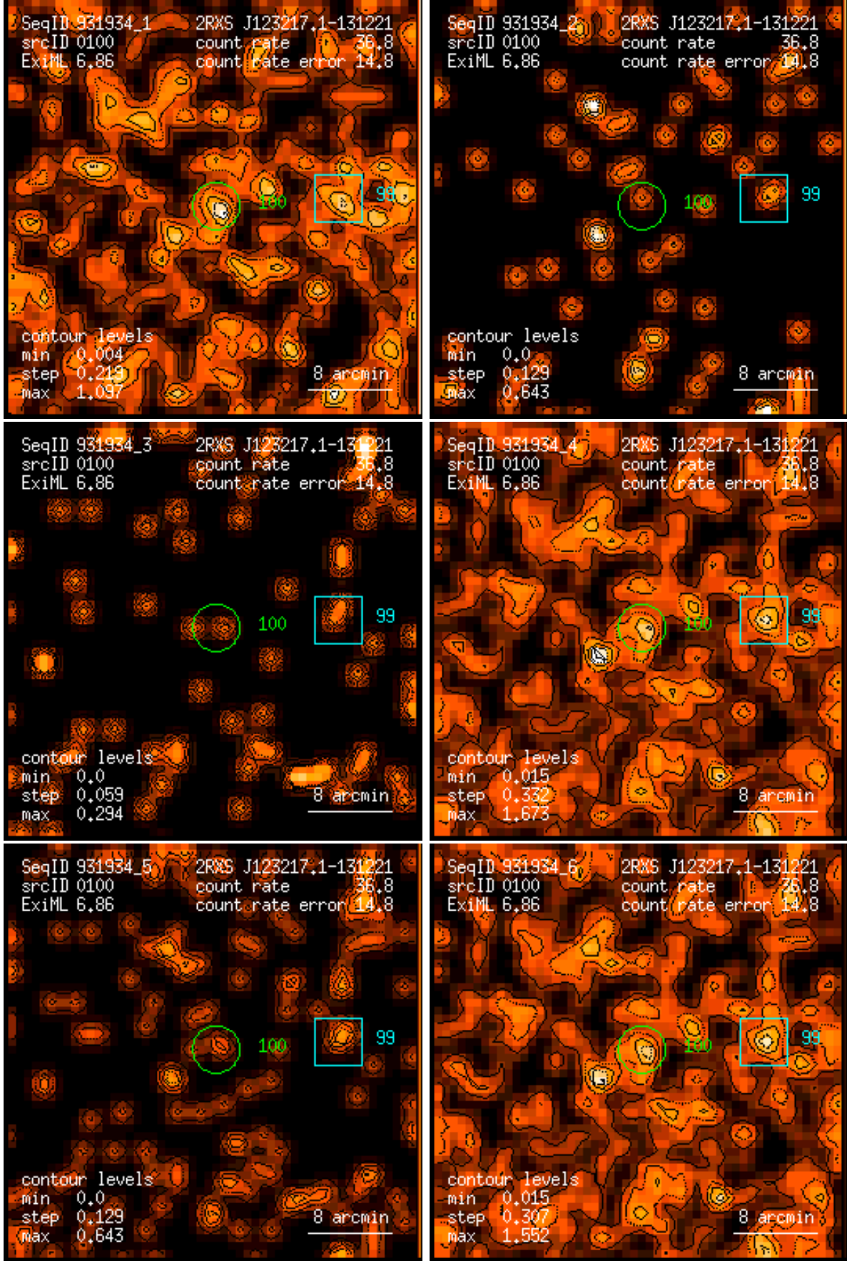
Figure 100: RASS 931934: detection 0100: band rate images, Gaussian filter: (1) PSPC channels 11 – 41, (2) 52 – 90, (3) 91 – 201, (4) 11 – 235, (5) 52 – 201, (6) 11 – 201. Broad band rates in counts/ks. Band rate contour levels in counts/ks/arcmin 2 .
