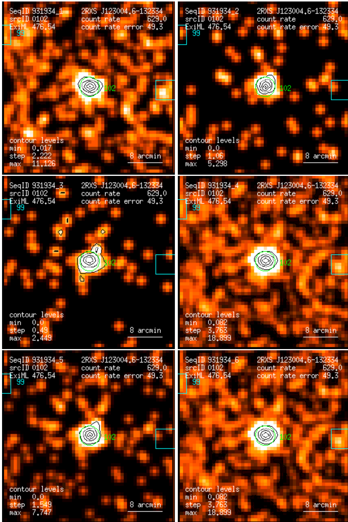
Figure 102: RASS 931934: detection 0102: band rate images, Gaussian filter: (1) PSPC channels 11 – 41, (2) 52 – 90, (3) 91 – 201, (4) 11 – 235, (5) 52 – 201, (6) 11 – 201. Broad band rates in counts/ks. Band rate contour levels in counts/ks/arcmin 2 .
