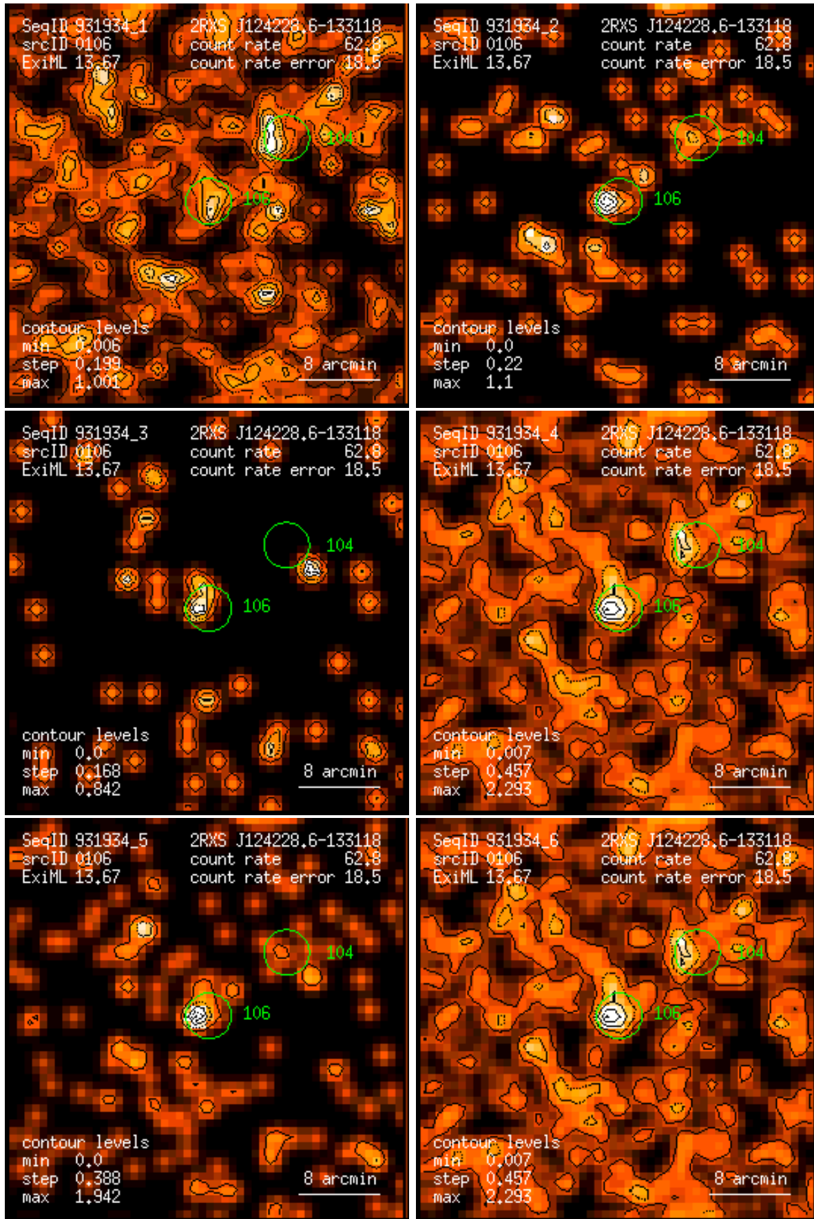
Figure 106: RASS 931934: detection 0106: band rate images, Gaussian filter: (1) PSPC channels 11 – 41, (2) 52 – 90, (3) 91 – 201, (4) 11 – 235, (5) 52 – 201, (6) 11 – 201. Broad band rates in counts/ks. Band rate contour levels in counts/ks/arcmin 2 .
