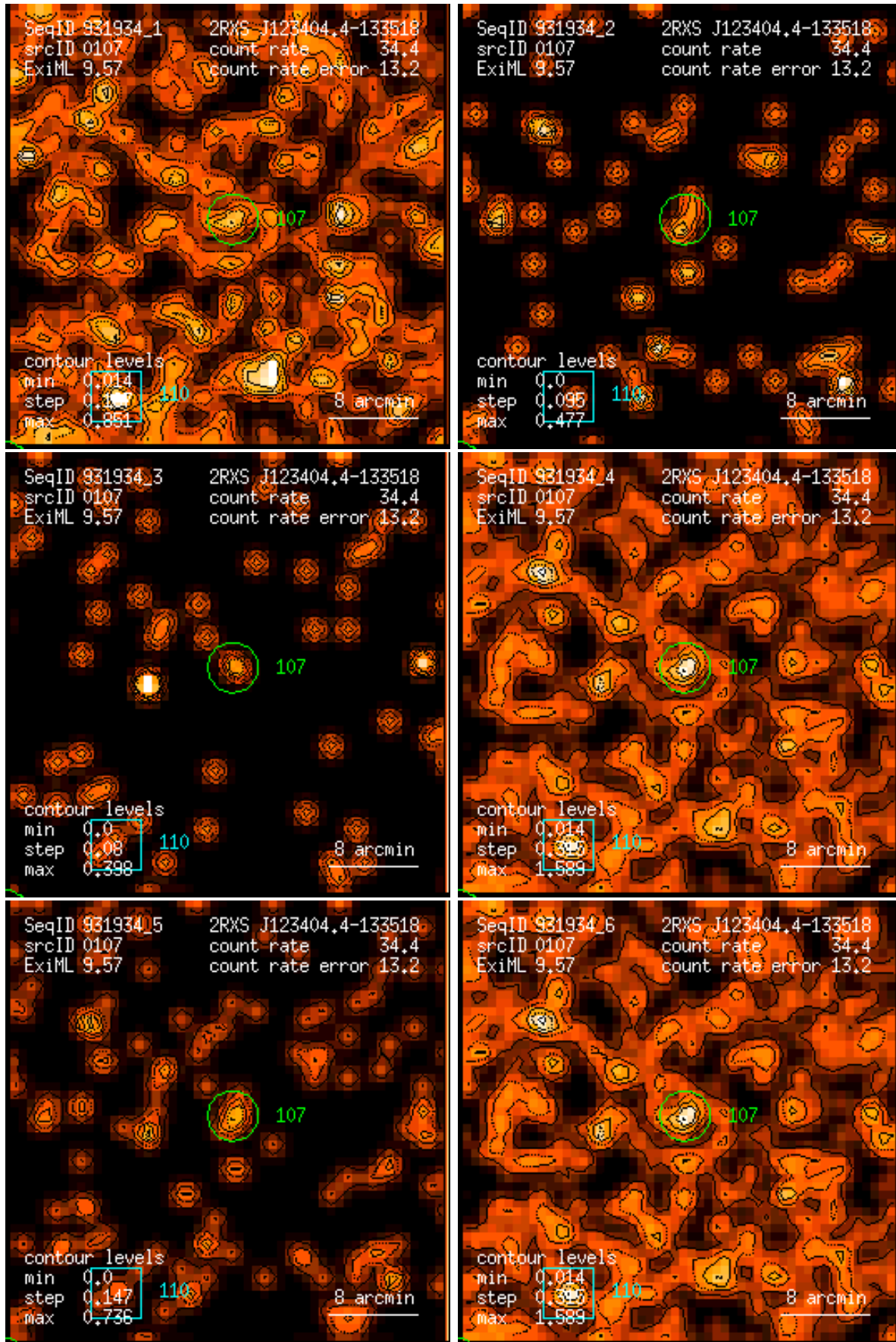
Figure 107: RASS 931934: detection 0107: band rate images, Gaussian filter: (1) PSPC channels 11 – 41, (2) 52 – 90, (3) 91 – 201, (4) 11 – 235, (5) 52 – 201, (6) 11 – 201. Broad band rates in counts/ks. Band rate contour levels in counts/ks/arcmin 2 .
