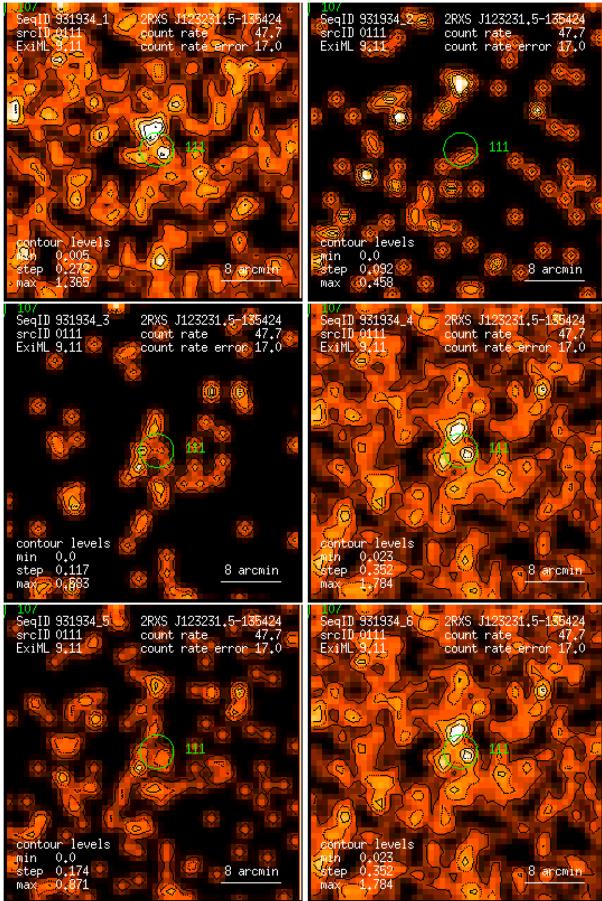
Figure 111: RASS 931934: detection 0111: band rate images, Gaussian filter: (1) PSPC channels 11 – 41, (2) 52 – 90, (3) 91 – 201, (4) 11 – 235, (5) 52 – 201, (6) 11 – 201. Broad band rates in counts/ks. Band rate contour levels in counts/ks/arcmin 2 .
