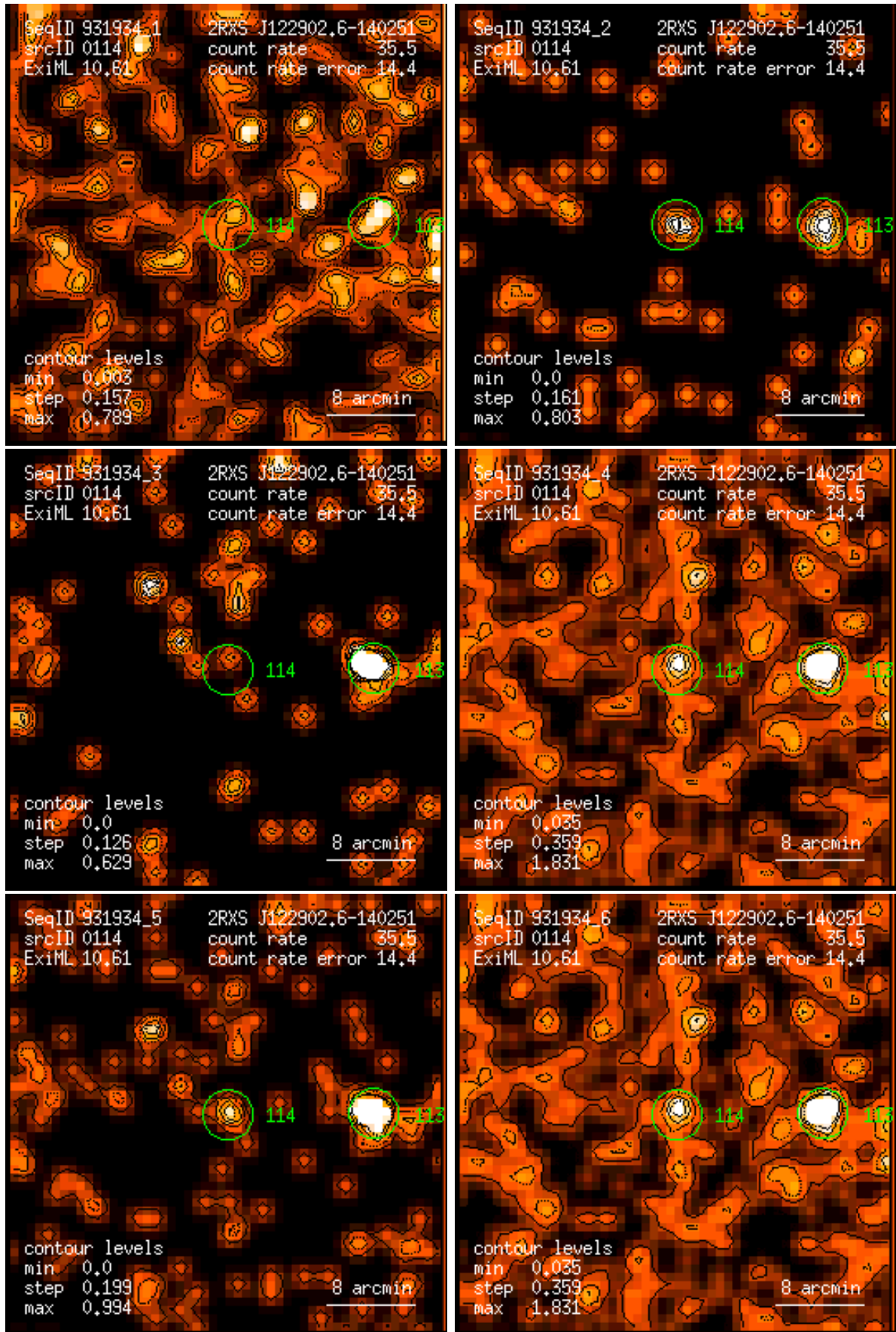
Figure 114: RASS 931934: detection 0114: band rate images, Gaussian filter: (1) PSPC channels 11 – 41, (2) 52 – 90, (3) 91 – 201, (4) 11 – 235, (5) 52 – 201, (6) 11 – 201. Broad band rates in counts/ks. Band rate contour levels in counts/ks/arcmin 2 .
