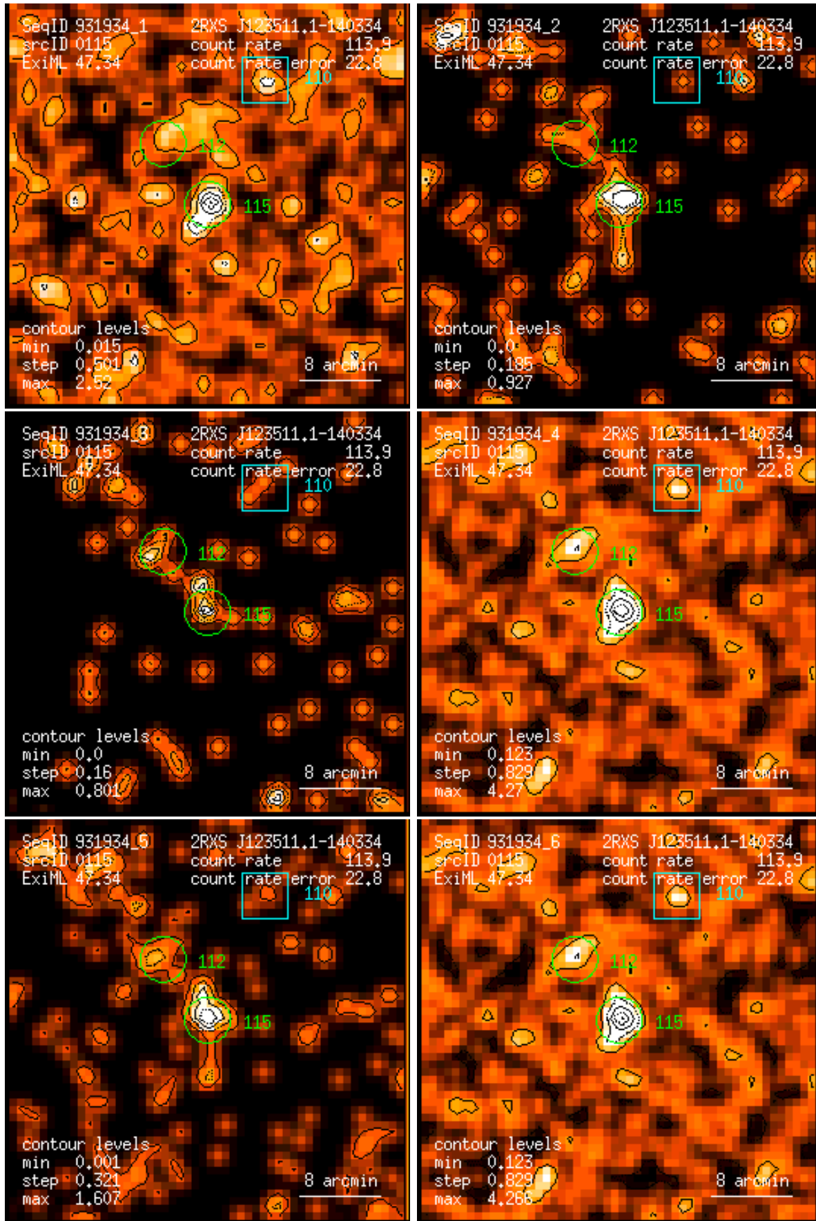
Figure 115: RASS 931934: detection 0115: band rate images, Gaussian filter: (1) PSPC channels 11 – 41, (2) 52 – 90, (3) 91 – 201, (4) 11 – 235, (5) 52 – 201, (6) 11 – 201. Broad band rates in counts/ks. Band rate contour levels in counts/ks/arcmin 2 .
