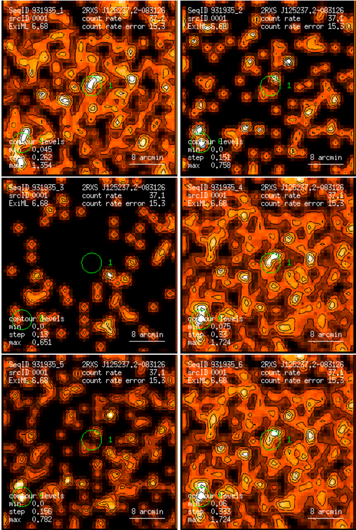
Figure 1: RASS 931935: detection 0001: band rate images, Gaussian filter: (1) PSPC channels 11 – 41, (2) 52 – 90, (3) 91 – 201, (4) 11 – 235, (5) 52 – 201, (6) 11 – 201. Broad band rates in counts/ks. Band rate contour levels in counts/ks/arcmin 2 .
