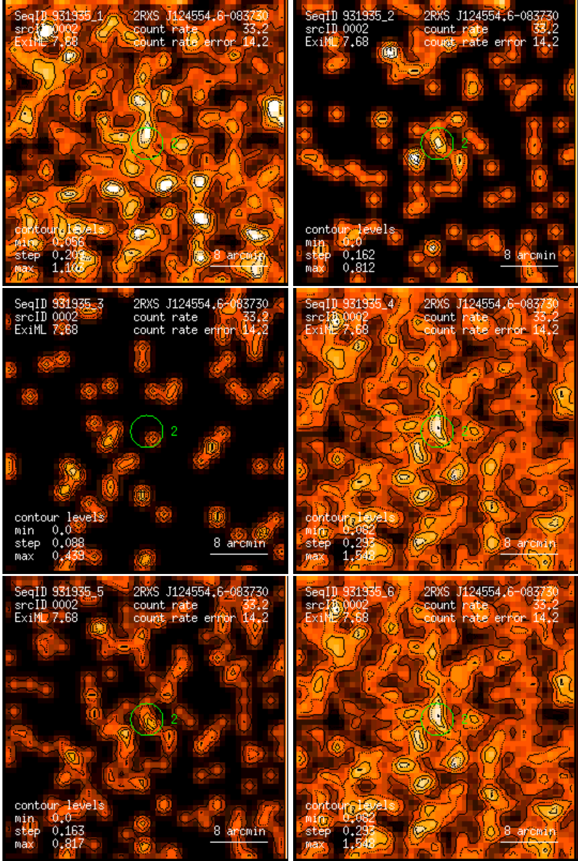
Figure 2: RASS 931935: detection 0002: band rate images, Gaussian filter: (1) PSPC channels 11 – 41, (2) 52 – 90, (3) 91 – 201, (4) 11 – 235, (5) 52 – 201, (6) 11 – 201. Broad band rates in counts/ks. Band rate contour levels in counts/ks/arcmin 2 .
