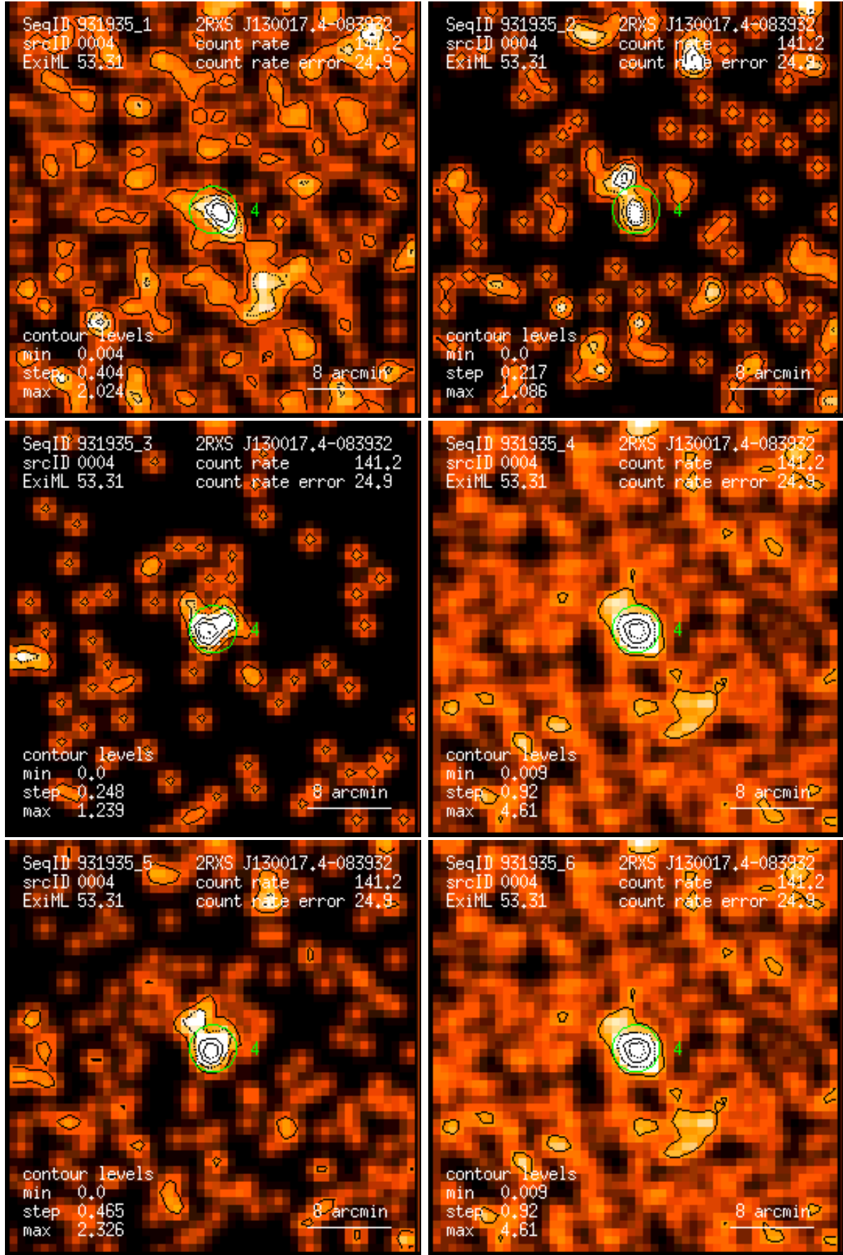
Figure 4: RASS 931935: detection 0004: band rate images, Gaussian filter: (1) PSPC channels 11 – 41, (2) 52 – 90, (3) 91 – 201, (4) 11 – 235, (5) 52 – 201, (6) 11 – 201. Broad band rates in counts/ks. Band rate contour levels in counts/ks/arcmin 2 .
